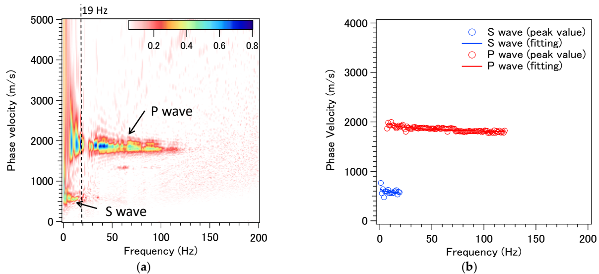
Figure 15. Velocity–frequency map (a) and dispersion curve (b).
