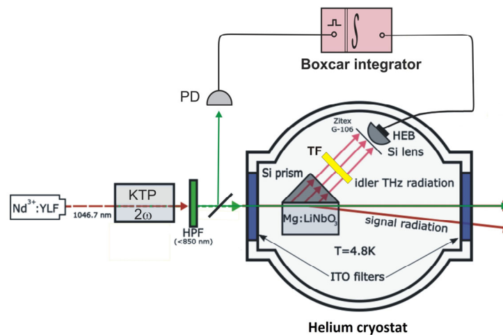
Figure 1. Schematics of the experimental set-up. The pumping radiation for PDC is generated using a series of the pulsed laser (Nd 3+ :YLF), the frequency doubling crystal (KTP), and the 1st harmonic cut-off filter (HPF). A small part of the pump beam is diverted by a mirror to a PIN diode (PD) which triggers integrator and boxcar averager modules SR250 (Boxcar integrator) at the beginning of each laser pulse. PDC originates in Mg-doped lithium niobate crystal (Mg:LiNbO 3 ) equipped by a prism from high-resistivity silicon (Si prism). The crystal and a system for detecting idler THz radiation are placed inside a He cryostat. The detection system contains a pump cut-off filter film (Zitex G-106), a narrow THz band pass filter Tydex BPF1.0-24/31 (TF), a focusing Si hemispherical lens (Si lens), and the NbN superconducting bolometer SCONTEL (HEB). The optical photons (signal radiation) are generated at small angles to the pump beam and leave the cryostat via the same windows as the pump radiation passes (marked by the blue color). In each window there is an external glass filter and an internal ITO filter. The latter is kept at the same temperature as the crystal and HEB.
