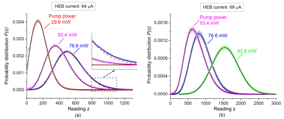
Figure 2. Histograms of the HEB detector readings, recorded experimentally under different laser pump powers (circles), and results of their numerical modeling (curves). The time-averaged pump power was 29.6 mW (red circles), 53.4 mW (magenta circles), 76.6 mW (blue circles), and 92.8 mW (green circles). The transport current of HEB was 64 \mu\text{A} (a) and 69 \mu\text{A} (b). Solid curves: numerical approximation by Equation (7). A dashed curve (a): approximation by Equation (6); the inset shows a plot section in an enlarged scale.
