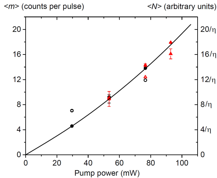
Figure 3. The mean number of the bolometer photo counts per pulse (in absolute unites, dots), and the theoretical prediction for the mean number of incident photons (in arbitrary units, a solid curve), both versus the time-averaged pump power. Open dots: results of approximation of experimental histograms by Equation (6), filled dots: by Equation (7). Black circular dots correspond to experimental data obtained under the HEB transport current of 64 \mu\text{A} , red triangular dots correspond to the data under the HEB transport current of 69 \mu\text{A} .
