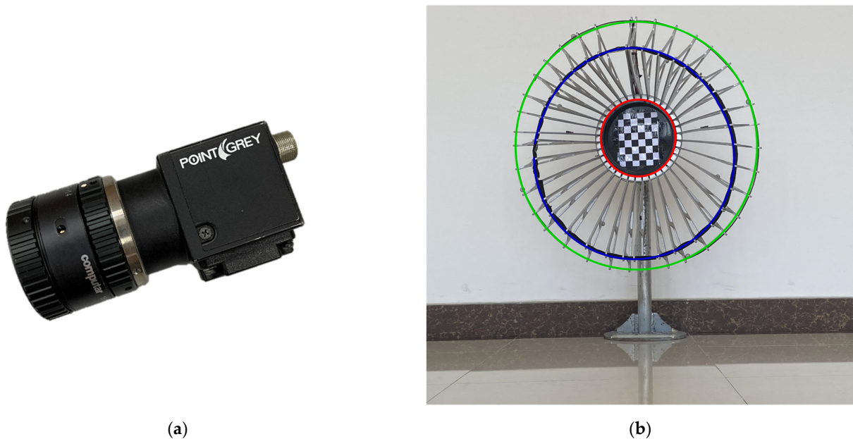
Figure 9. This is a figure about the experimental equipment. (a) A photo of the camera and the lens used for image capture. (b) A photo of the drogue model.
