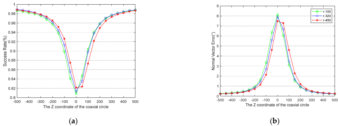
Figure 7. This is a figure about the relationship between the performance of the proposed algorithm and the target's spatial structure when the z-axis coordinate of the target is 7 m. (a) The curves of the success rate. (b) The curves of the normal vector's angle error.
