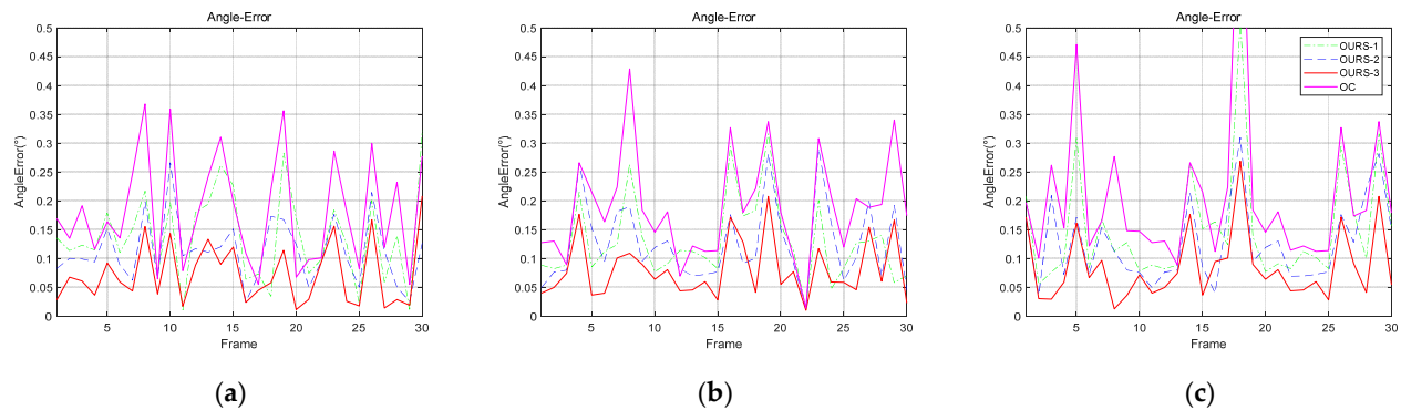
Figure 5. This is a figure showing some examples of simulations for the angle error of the normal vector. (a) The angle error of the normal vector when the variance in the image feature noise is 2; (b) The angle error of the normal vector when the variance in the spatial structure noise is 20; (c) The angle error of the normal vector at z-axis coordinates of 6 m.
