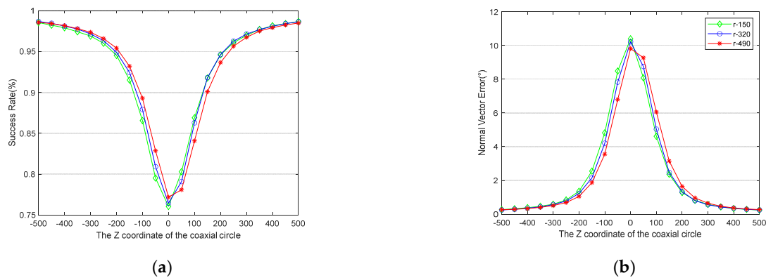
Figure 8. This is a figure about the relationship between the performance of the proposed algorithm and the target's spatial structure when the z-axis coordinate of the drogue is 9 m. (a) The curves of the success rate. (b) The curves of the normal vector's angle error.
