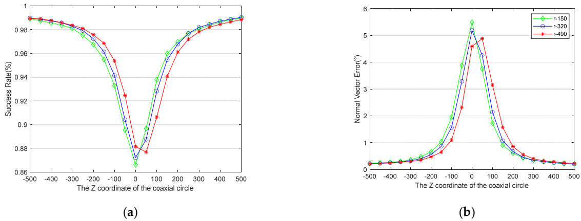
Figure 6. This is a figure about the relationship between the performance of the proposed algorithm and the target's spatial structure when the z-axis coordinate of the target is 5 m. The curves of the different radii are marked r-150, r-320, and r-490, respectively. (a) The curves of the success rate. (b) The curves of the normal vector's angle error.
