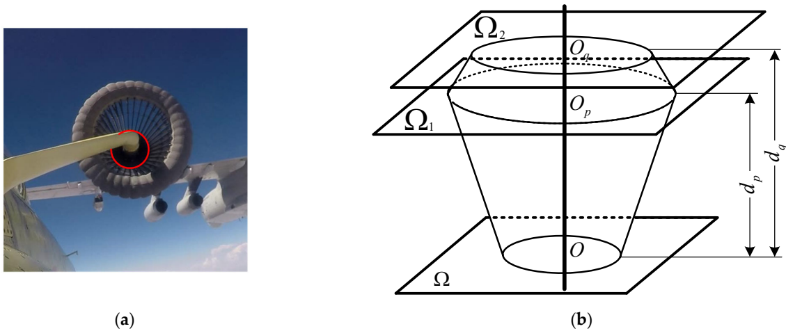
Figure 1. This is a figure of a drogue for aerial refueling. (a) The drogue during aerial refueling seen from the perspective of the receiver; (b) a side view of the drogue model.
