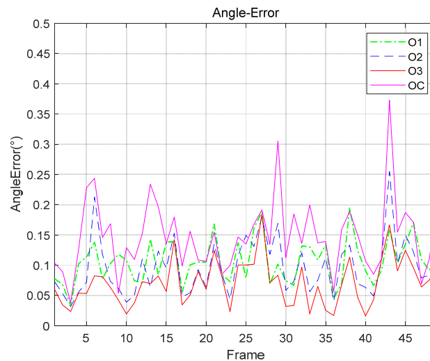
Figure 10. This is a figure of the angle error of the normal vector corresponding to the captured images.
