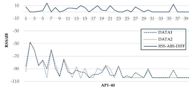
Figure 2. RSS difference of part AP (AP1–AP40) at the same position.
