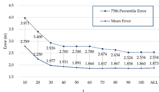
Figure 8. Positioning errors of different L on Zenodo.
