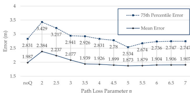
Figure 7. Positioning errors of different values of \eta on Zenodo.
