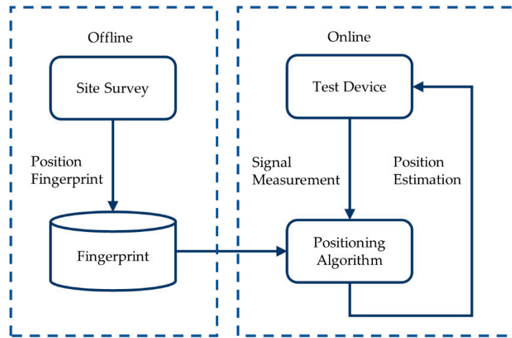
Figure 1. Flowchart of fingerprint positioning algorithm.
