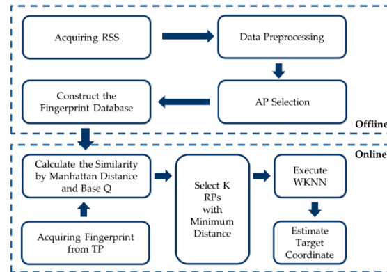
Figure 3. Flowchart of proposed algorithm.
