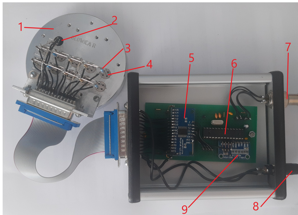
Figure 1. The PW6 electronic nose device. The cover was opened for the photo. 1 – aluminium probe, 2 – temperature and humidity sensors, 3 – additional resistor, 4 – TGS sensor, 5 – 16-channel analogue multiplexer (Texas Instruments, Dallas, TX, USA), 6 – Atmel 0814G Atmega 8-16PU microcontroller (Microchip Technology, Chandler, AZ, USA), 7 – USB wire, 8 – external power supply wire, 9 – 16-bit ADS1115 AD converter Texas Instruments, Dallas, TX, USA).
