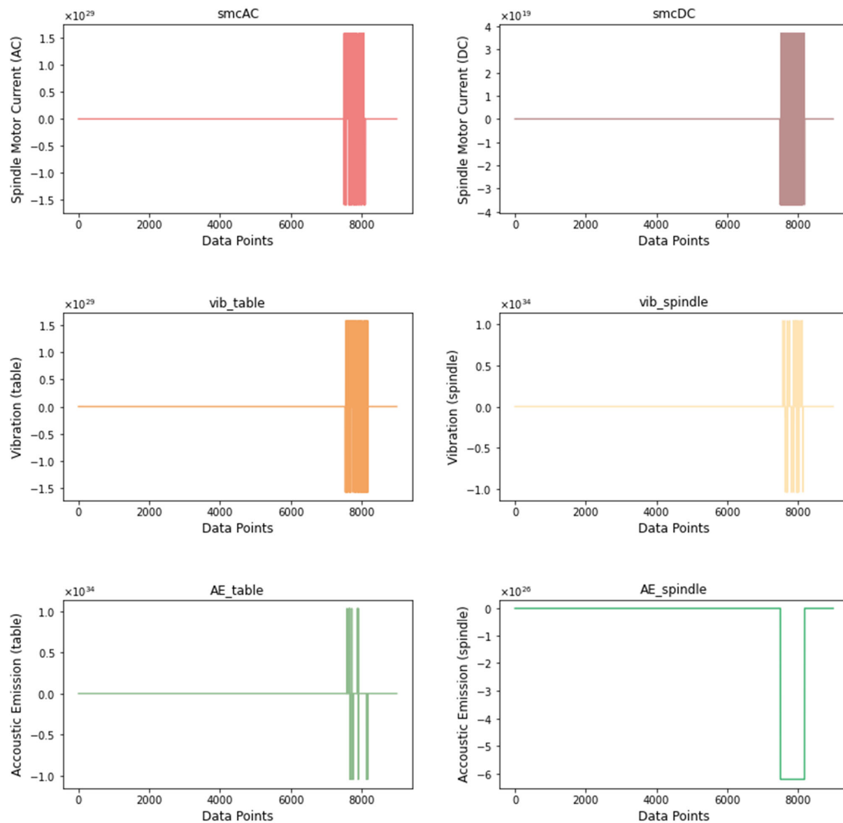
Figure 4. Signatures from the six sensors showing an outlier for case 2, run 1.
