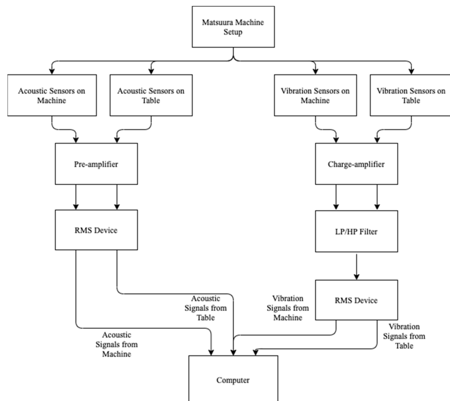
Figure 3. Milling operation setup, adapted from [79].
