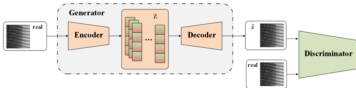
Figure 4. Structure of basic reconstruction GAN.
