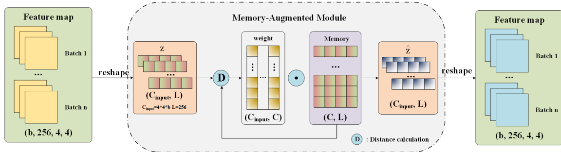
Figure 6. Details of the memory-augmented module.
