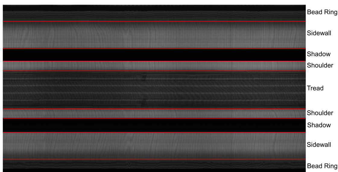
Figure 2. A horizontally displayed entire defect-free X-ray image, divided into five areas: bead ring, sidewall, shadow, shoulder and tread.
