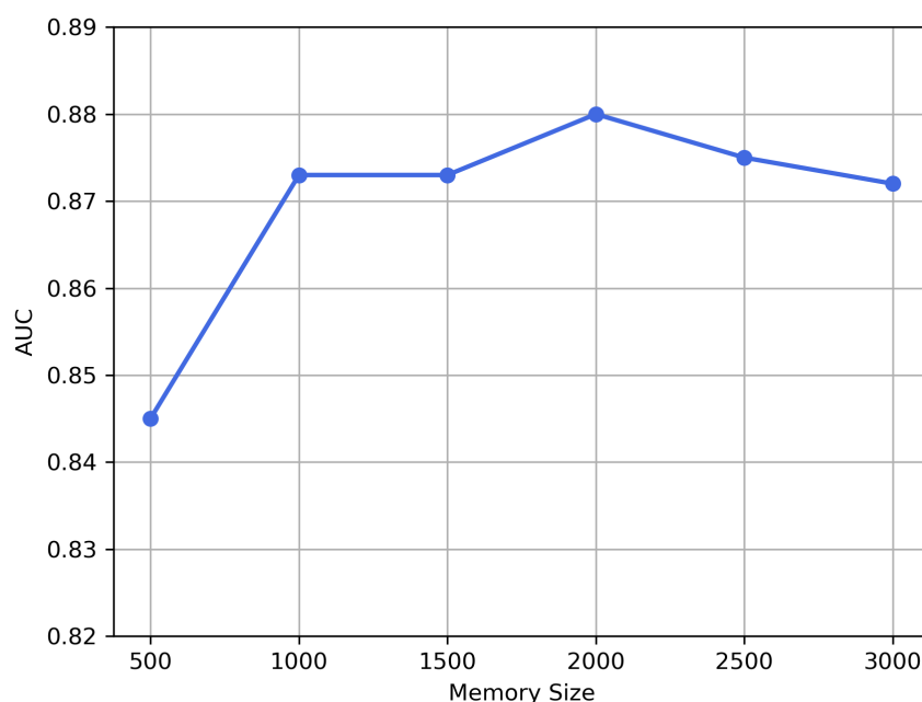
Figure 10. Impact of the size of memory on AUC.
