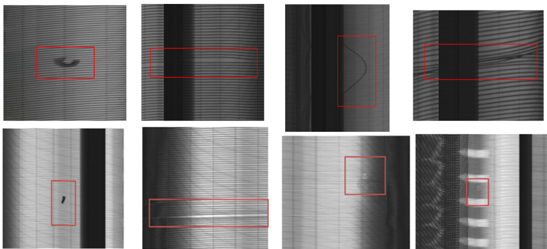
Figure 3. Typical defects in tire X-ray images.
