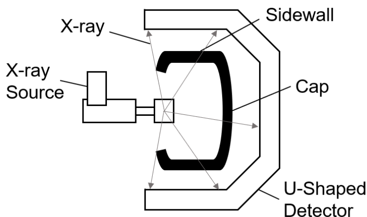
Figure 1. How the imaging equipment works.
