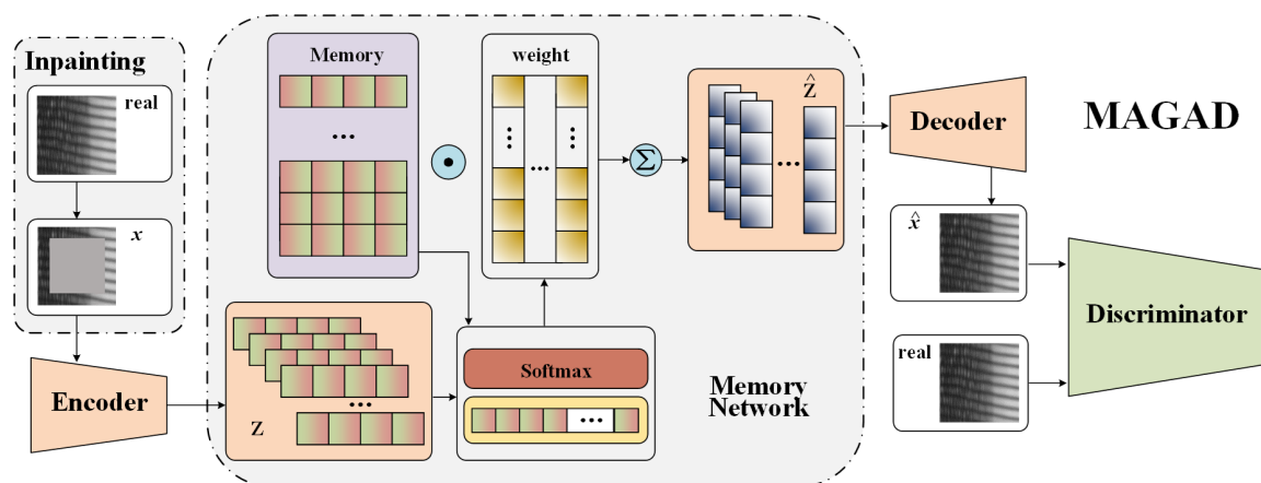
Figure 5. Structure of MAGAD.
