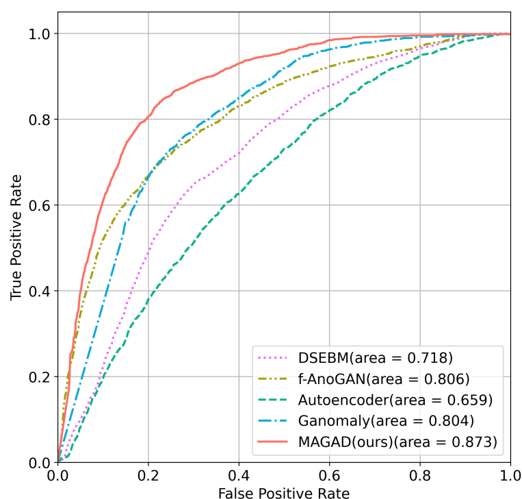
Figure 9. Comparison of ROC curves among five models.
