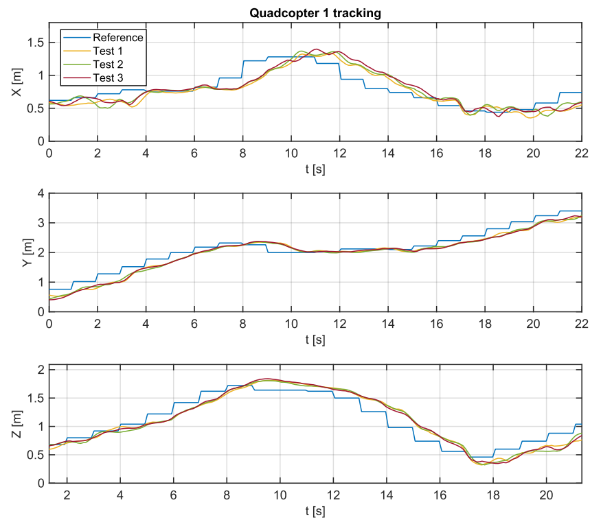
Figure 8. Path tracking of UAV 1.
