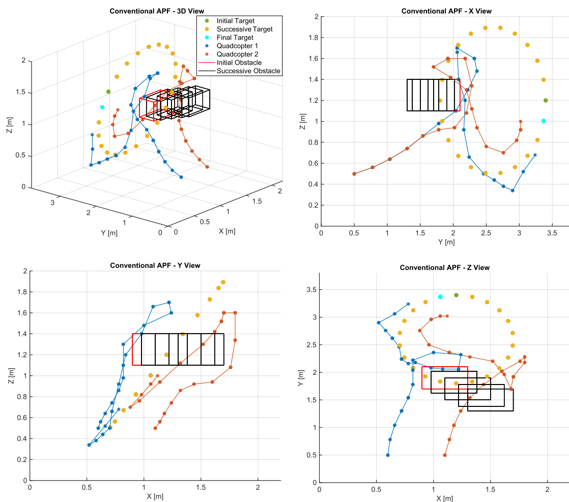
Figure 5. Paths calculated by the conventional APF algorithm.
