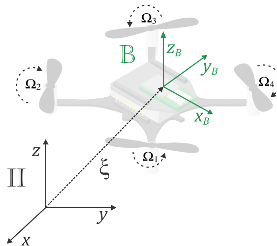
Figure 1. Coordinate systems of a quadrotor.
