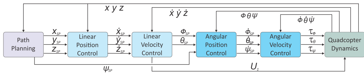
Figure 2. Information flow of the cascade controller.
