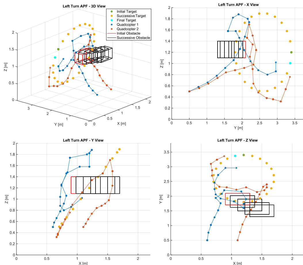
Figure 6. Paths calculated by the LTAPF algorithm.
