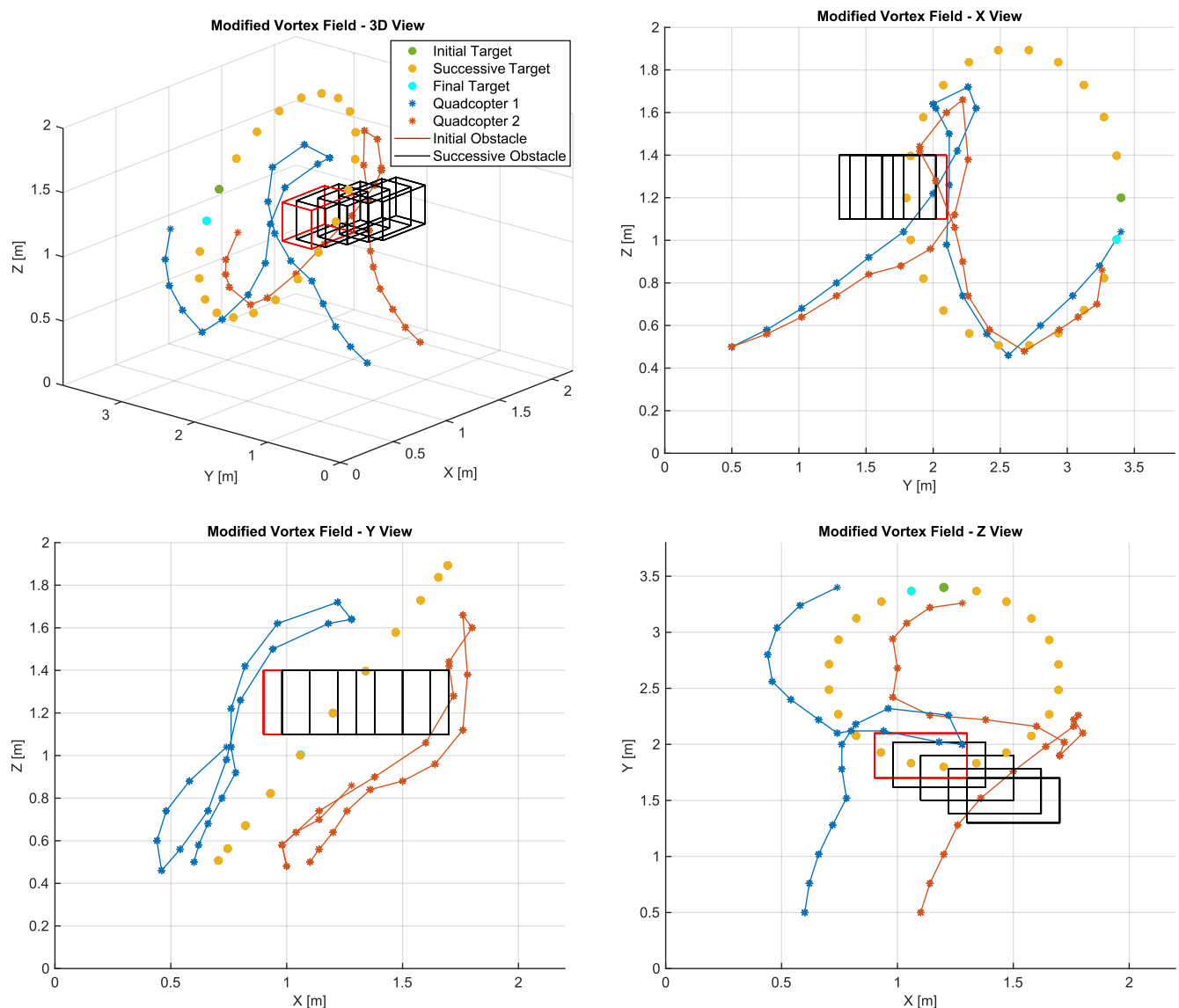
Figure 7. Path calculated by the proposed vortex field APF.
