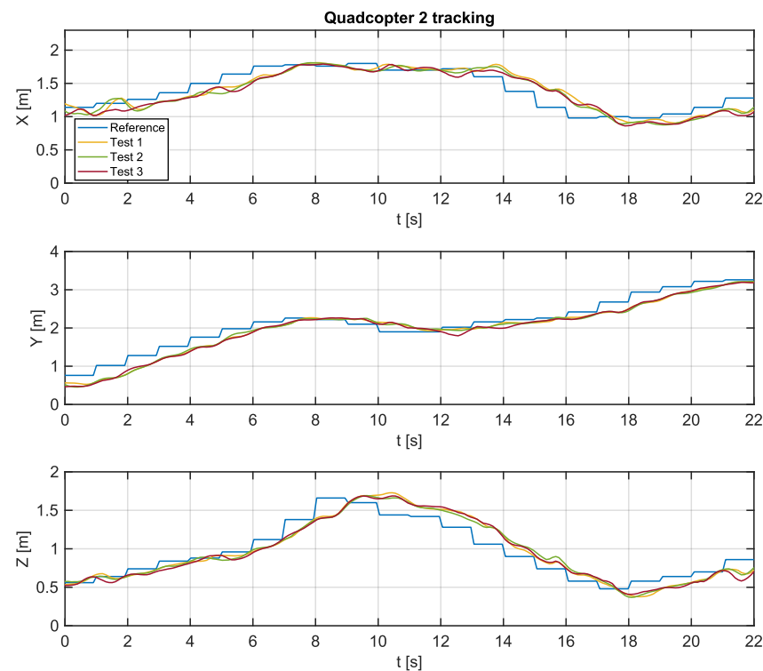
Figure 9. Path tracking of UAV 2.
