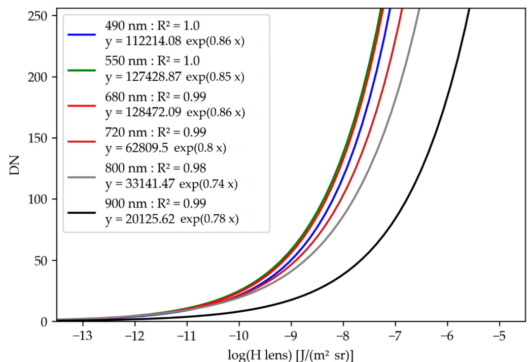
Figure 4. Response curves of the monochrome cameras. Each camera is designated using the central wavelength of the narrow-band optical filter. The response curves model the relation between image digital numbers (DNs) and exposure at camera lens ( H_{\text{lens}} ).
