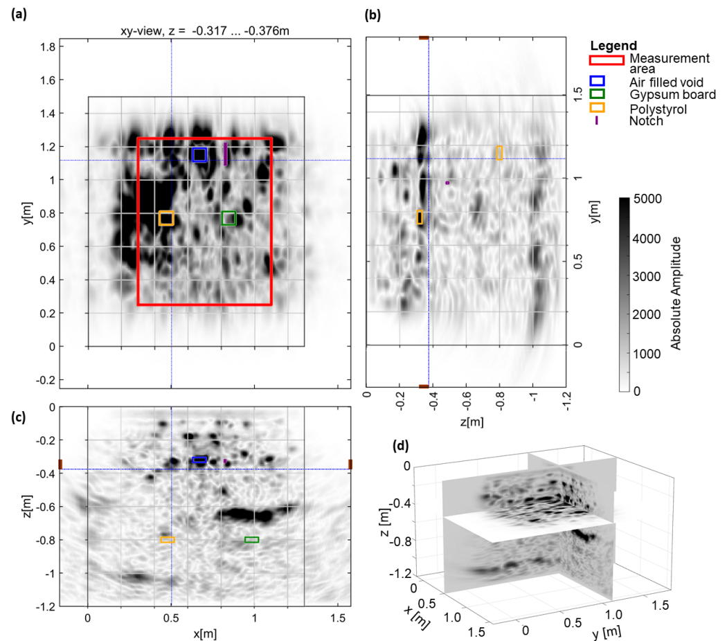
Figure 9. Ultrasonic imaging results of GSBV4 overlain by expected location of artificial defects (compare Figure 8): (a) xy-slice at z = -0.32 m, (b) yz-slice, (c) xz-slice, and (d) 3D view at marked slices.
