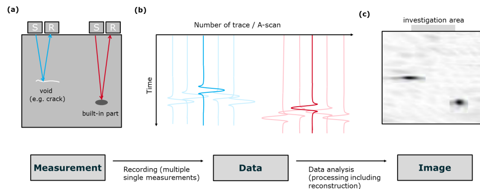
Figure 2. Summary of the applied ultrasonic echo method: (a) measurements with sender/receiver pair, (b) data represented in the time/space domain, (c) reconstructed ultrasonic image in the depth/space domain.
