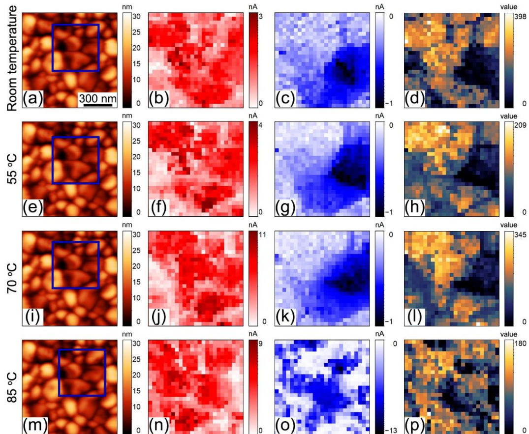
Figure 4. IV dependencies mapping at various temperatures: (a–d) 25\ ^\circ\text{C} , (e–h) 55\ ^\circ\text{C} , (i–l) 70\ ^\circ\text{C} , (m–p) 85\ ^\circ\text{C} . (a,e,i,m) Topography; current in log-scale (b,f,j,n) at U = 10\ \text{V} and (c,g,k,o) at U = -10\ \text{V} ; (d,h,l,p) coefficient of asymmetry: current amplitude at 10\ \text{V} divided on current amplitude at -10\ \text{V} . Thermal drift is present in (m–p). Blue squares in (a,e,i,m) indicate the region at the scan, where I–V curve mapping was done in the respective row.
