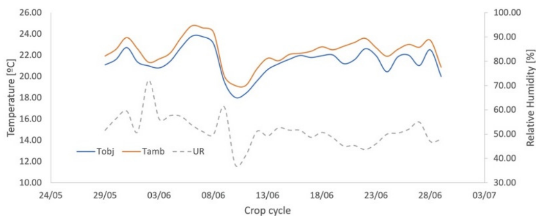
Figure 5. Ambient ( T_{amb} ) and Object Temperature ( T_{obj} ) monitoring and Relative Humidity (UR) for the auxiliary bench in NWSB parameterization.
