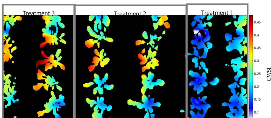
Figure 15. CWSI (Crop Water Stress Index) map generated for 25DAP (Day After Planting), using the empirical method to obtain the T_{UL} (Temperature Upper Limit) and T_{LLN} (Temperature Lower Limit) through natural reference surfaces. One of the leaves was wetted with water to simulate 100% transpiration and the other was covered with Vaseline to block leaf transpiration. Treatment 1 ( T_1 = 85% FC (Field Capacity)); Treatment 2 ( T_2 = 75% FC); Treatment 3 ( T_3 = 55% FC).
