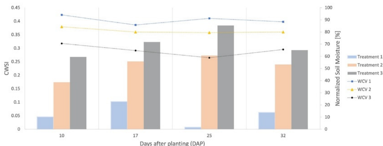
Figure 16. Levels of water stress throughout the entire arugula cycle. Soil moisture was normalized by the field capacity of each treatment, thus equaling the references used for measurement. CWSI
