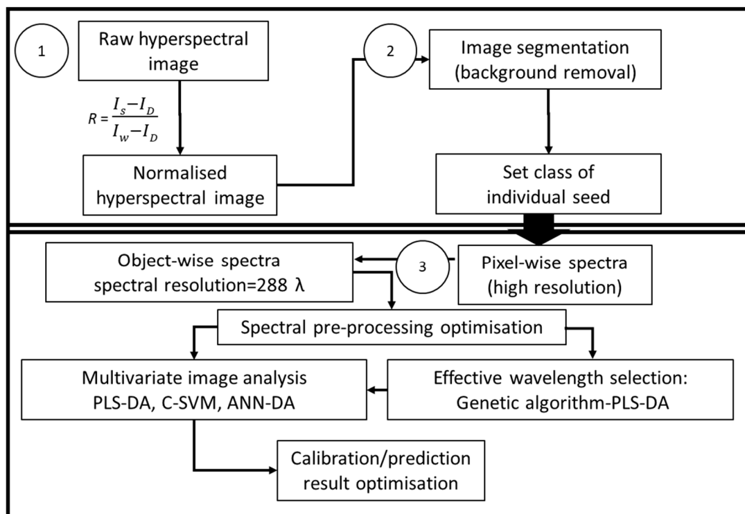
Figure 1. Flow chart of steps for analysing raw hyperspectral image of seeds. (1) Normalisation of image based on white and dark reference; (2) Image segmentation for background removal; (3) Spectral pre-processing and classification model development.
