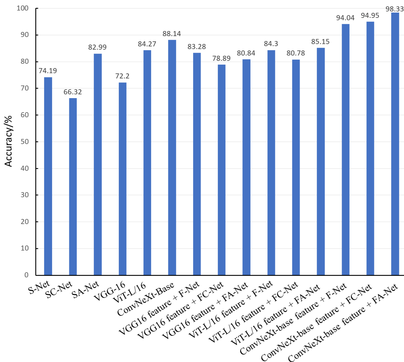
Figure 12. Comparison of the accuracy of pear leaf nutrient deficiency disease identification algorithms on the test set.
