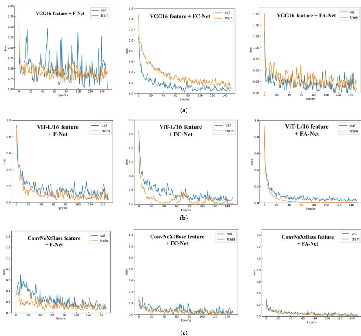
Figure 11. (a) Loss variation curve of the identification algorithm based on the VGG16 feature and shallow feature fusion. (b) Loss variation curve of the identification algorithm based on the ViT-L/16 feature and shallow feature fusion. (c) Loss variation curve of the identification algorithm based on the ConvNeXt-Base feature and shallow feature fusion.
