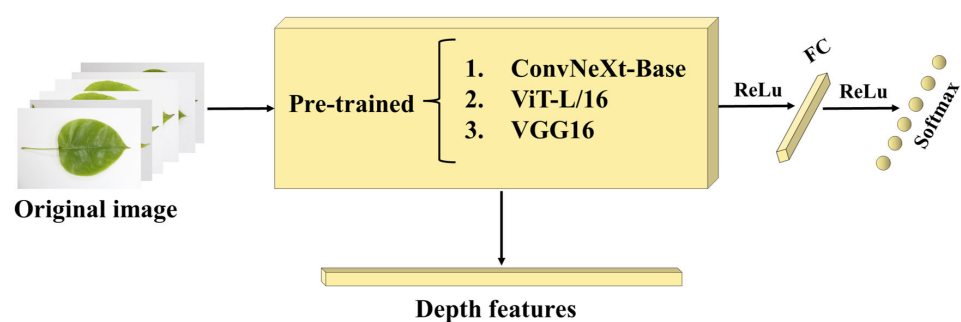
Figure 5. Flow chart of the depth feature-based identification algorithm.
