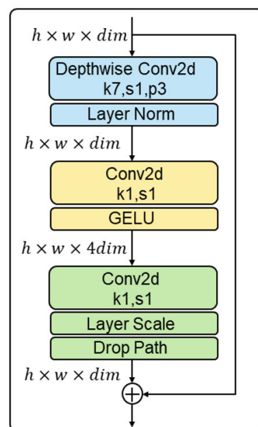
Figure 3. The block of ConvNeXt.
