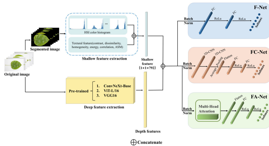
Figure 7. Flow chart of the identification algorithm based on depth feature and shallow feature fusion.
