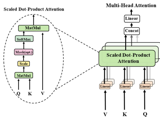
Figure 6. Multi-Head Attention consists of several attention layers running in parallel, which is a redrawn figure of Figure 2 from the cited paper [41].
