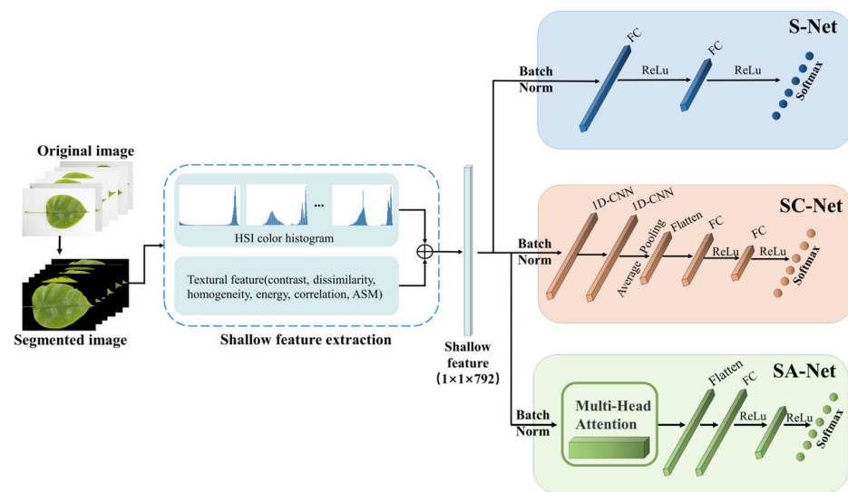
Figure 2. Flow chart of the shallow feature-based identification algorithm.
