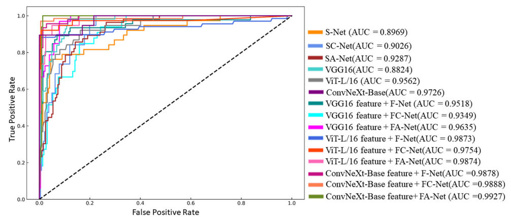
Figure 13. Receiver operating characteristic (ROC) curves of the pear nutrient deficiency disease identification algorithm.
