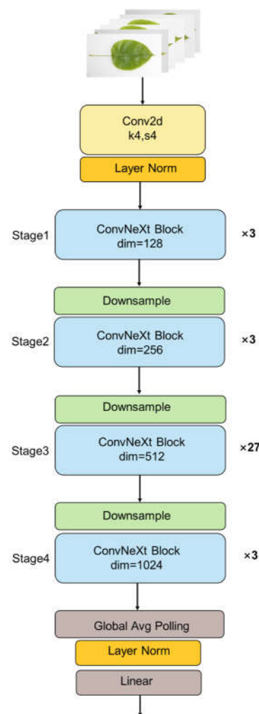
Figure 4. The structure of ConvNeXt-Base.
