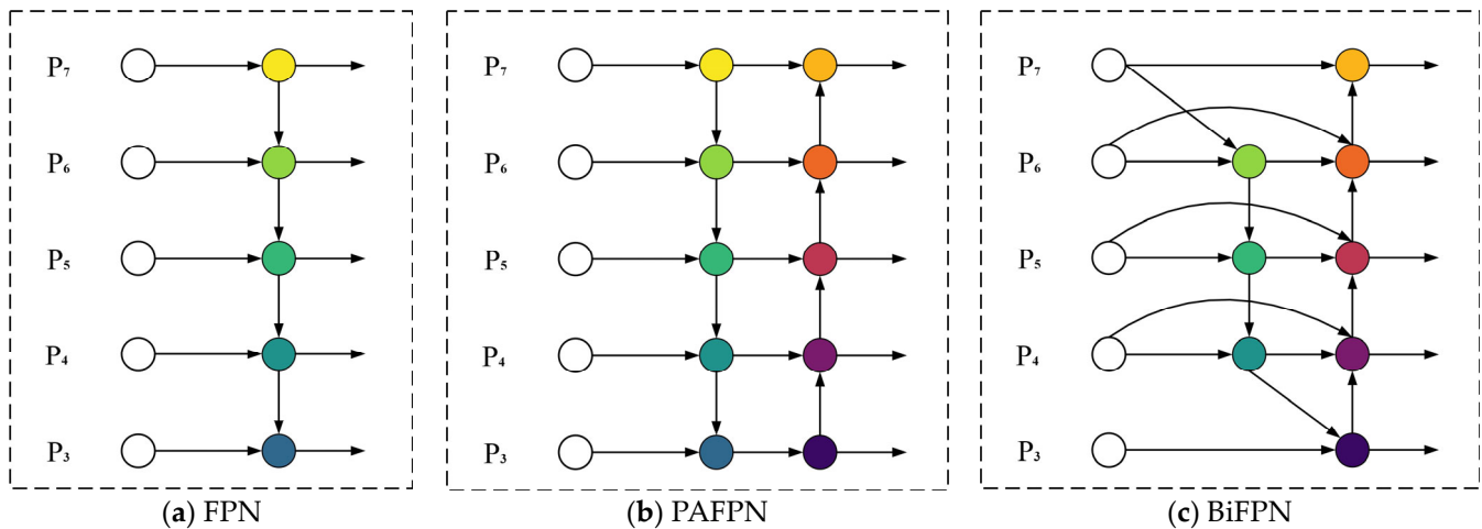
Figure 6. The architectures of different FPNs.
