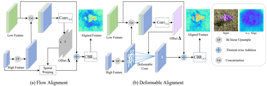
Figure 1. Illustration of various alignment technologies. \text{CBR}_{3 \times 3} means a 3 \times 3 convolution followed by batch normalization and ReLU operations. \text{Conv}_{3 \times 3} is a 3 \times 3 convolution to generate offset. The feature maps of each model are visualized by averaging along the channel dimension. Larger values are denoted by hot colors, and vice versa.
