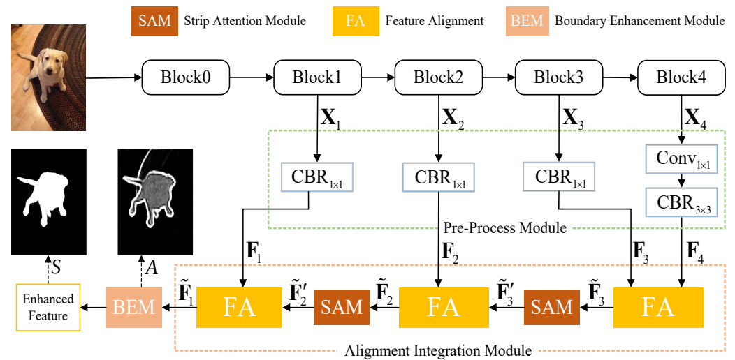
Figure 2. Main framework of our alignment integration network; CBR_{k \times k} means a k \times k convolution followed by batch normalization and ReLU operations. We first side-out the multi-level convolutional features from the backbone and process them by the pre-process module. An additional 3 \times 3 convolution operation is applied on the top level feature to encode high-level semantics. Then, features from multi-level are fed into the alignment integration module, in which adjacent level features are progressively combined by feature alignment. A strip attention module is utilized to capture non-local contextual information for the intermediate integrated feature. The final integrated feature is further enhanced by a boundary enhancement module, and the enhanced feature is exploited to conduct salient object prediction.
