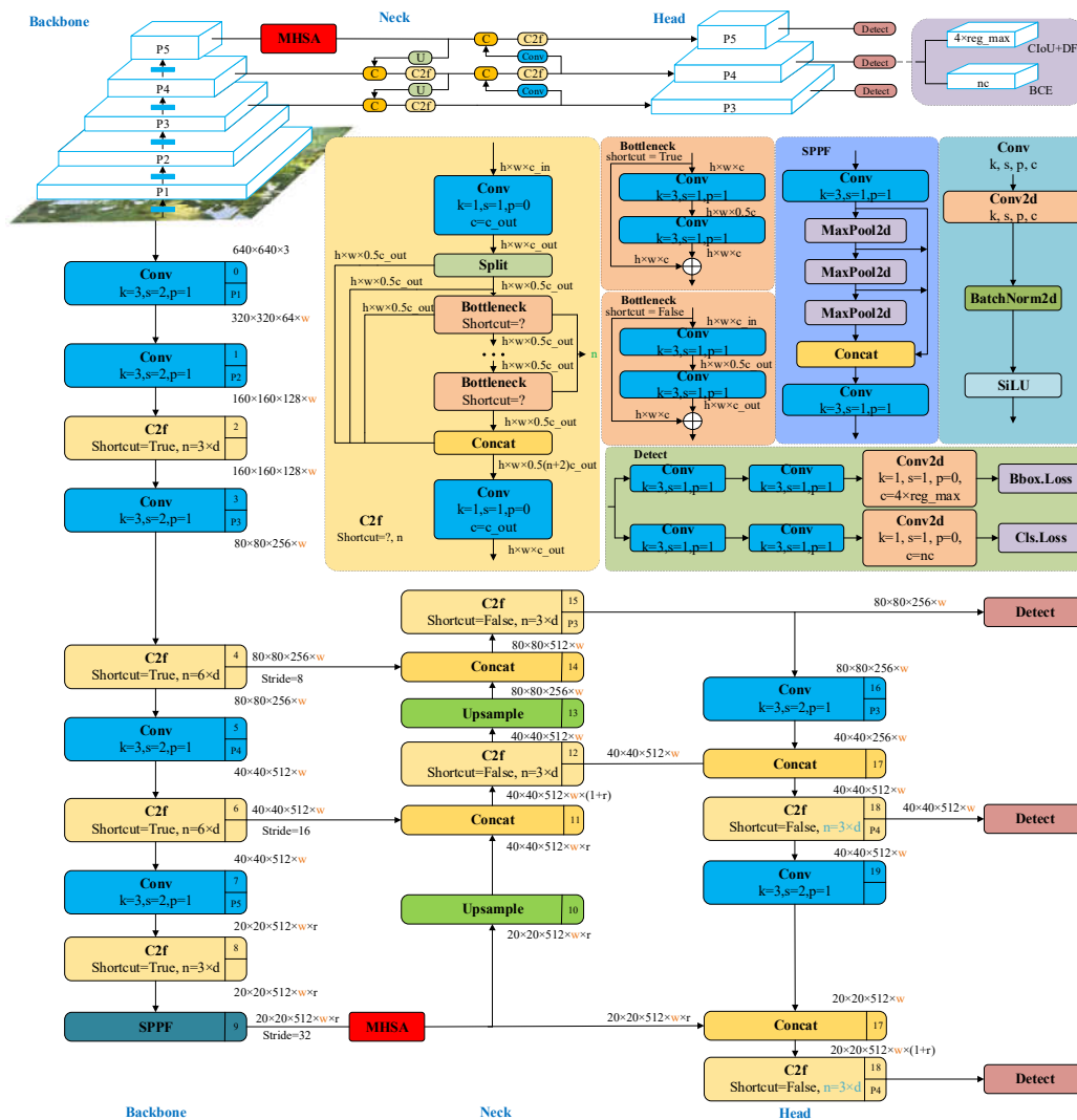
Figure 4. Network structure of MHA-YOLOV8. Among them, the black arrow represents the direction of data flow during network operations, and different colors represent different network modules. For example, blue represents convolutional modules and yellow represents C2f modules. The name of each module is located at the top left or bottom left of the rectangle where it is located.
