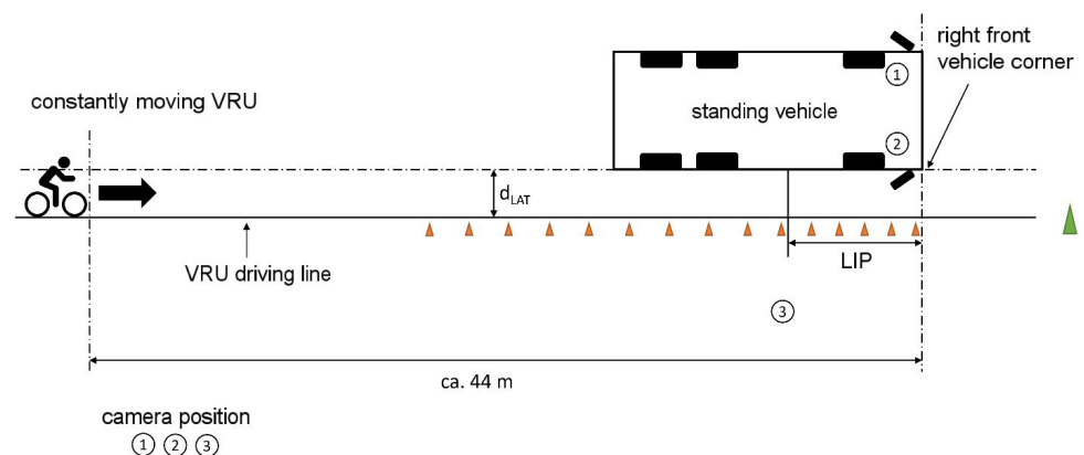
Figure 2. Static experimental setup with VRUs driving parallel to the commercial vehicle.
