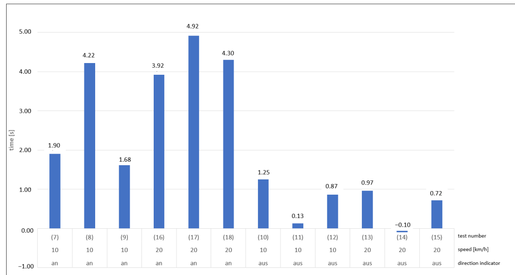
Figure 8. Remaining time between the occurrence of the acoustic warning signal and the theoretical collision.
