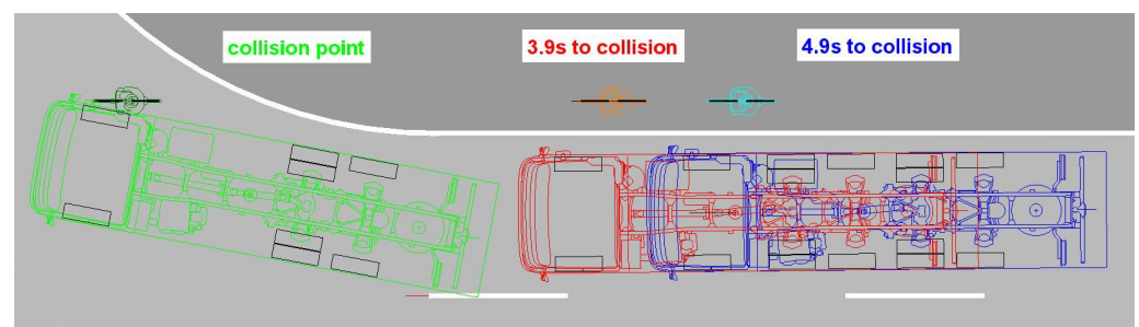
Figure 9. Shutter release range of the blind spot assistance system when the direction indicator is activated.
