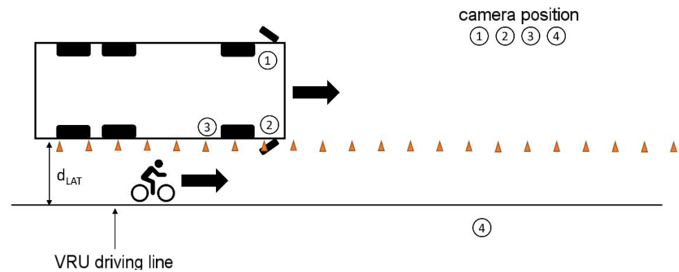
Figure 4. Dynamic test setup with parallel movement of commercial vehicle and VRU.
