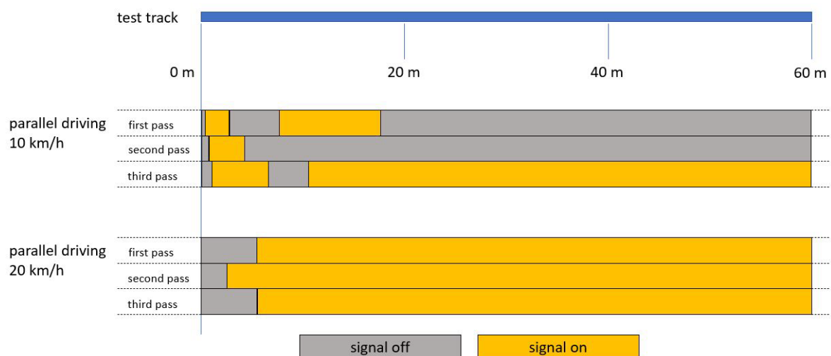
Figure 7. Time course of the information signal during tests in parallel travel at the same speed at a lateral distance of 1.25 m without visual obscuration.
