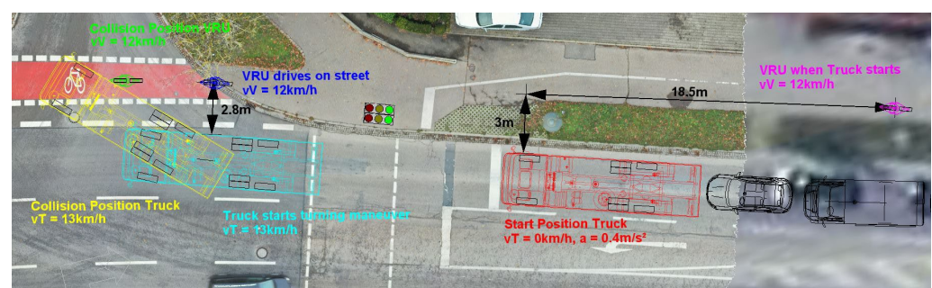
Figure 12. Typical accident between a VRU and a right-turning commercial vehicle.
