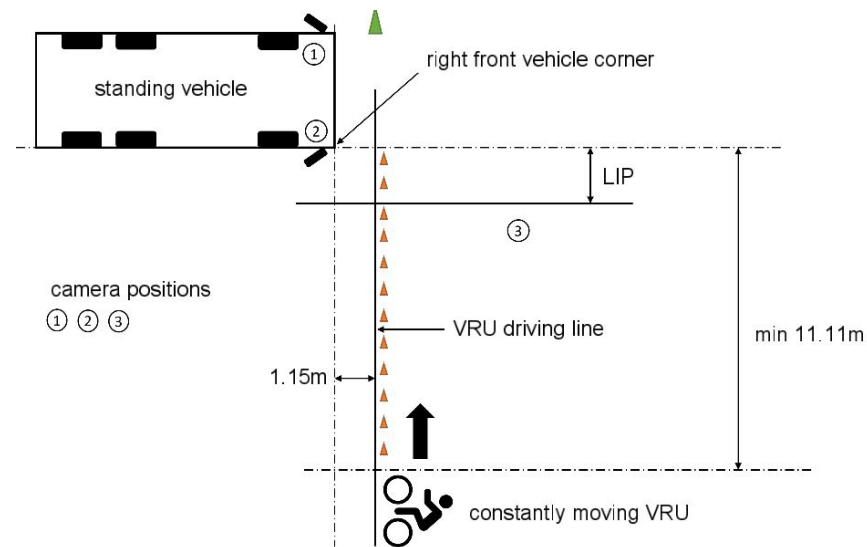
Figure 1. Static experimental setup with the VRU crossing the front of the commercial vehicle.
