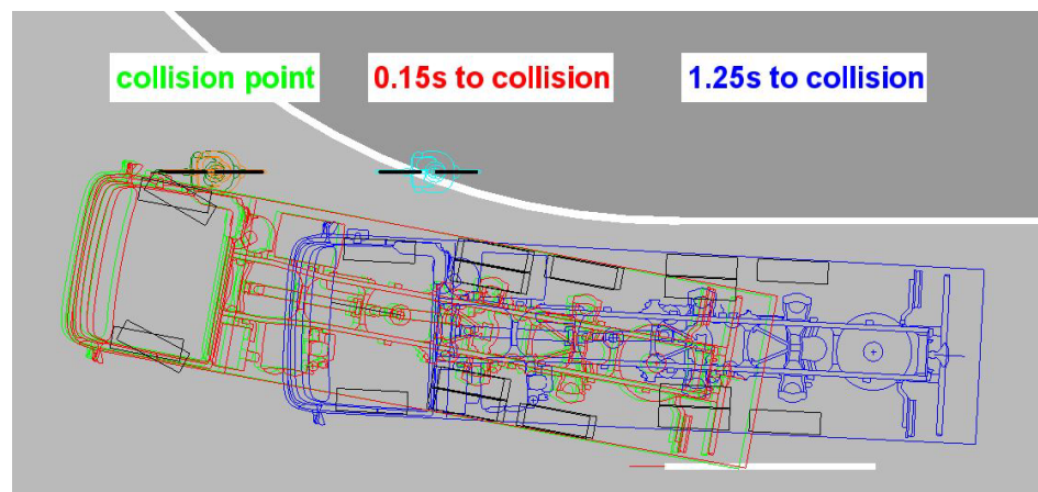
Figure 10. Blind spot assistance system triggering range without direction indicator activated.
