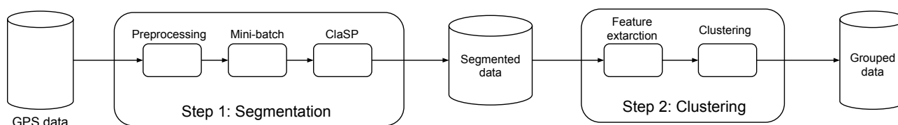
Figure 1. The proposed two-step analysis framework.
