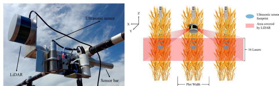
Figure 11. Phenotyping system and scanning areas of LiDAR and ultrasonic sensors [145].
