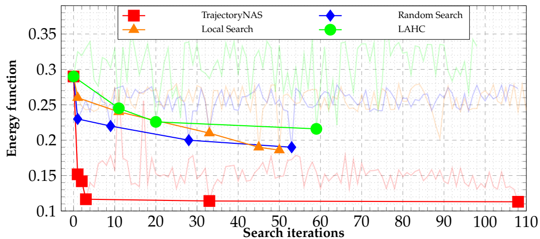
Figure 4. TrajectoryNAS optimization curve.
