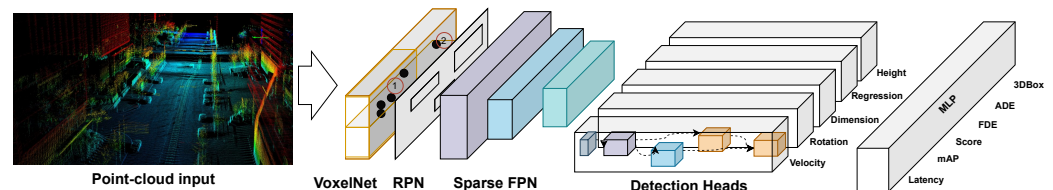
Figure 3. The overview of TrajectoryNAS process.
