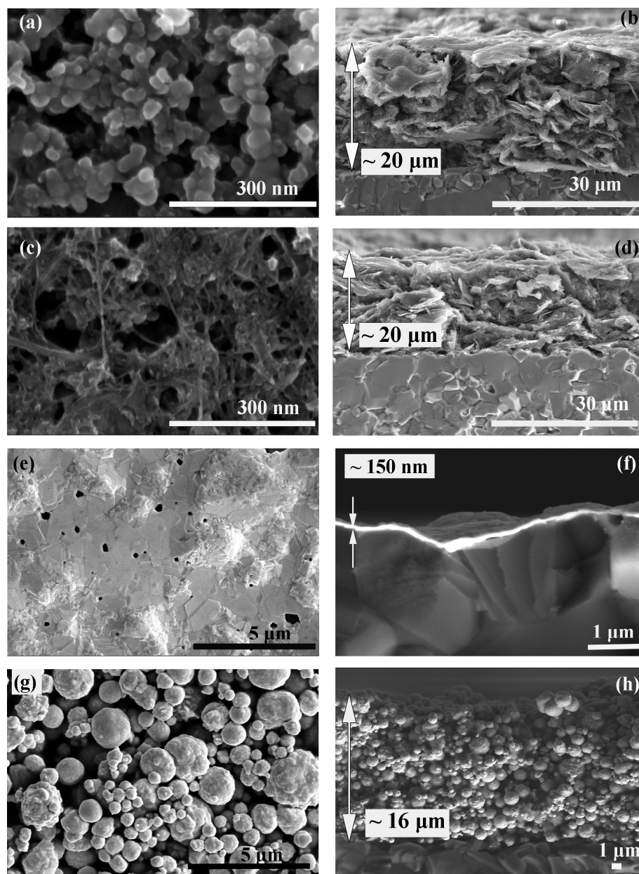
Figure 2. Top view and cross-section of: SPE-C (a,b), SPE-SWCNT (c,d), SPE-Au-AT (e,f) and SPE-Au-BT (g,h) electrodes.
