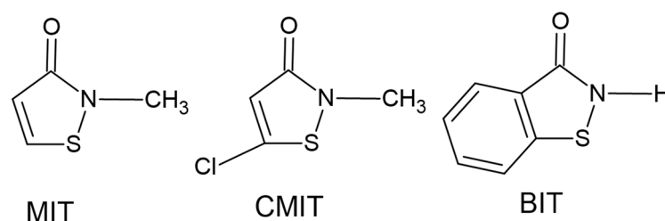
Figure 1. Chemical structures of the most used isothiazolinones: methylisothiazolinone (MIT), chloromethylisothiazolinone (CMIT), and benzisothiazolinone (BIT).
