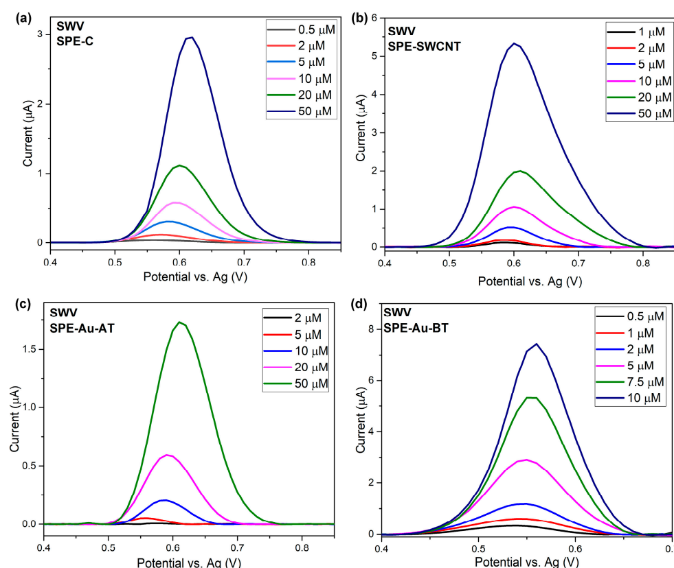
Figure 5. SWV voltammograms of BIT oxidation on (a) SPE-C, (b) SPE-SWCNT, (c) SPE-Au-AT and (d) SPE-Au-BT. Measurement parameters are presented in Table S1.
