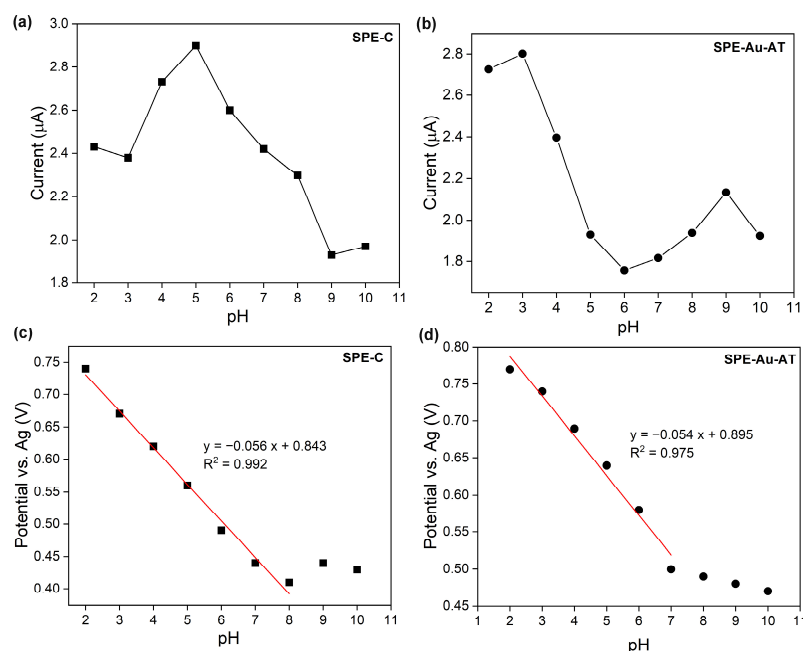
Figure 6. 50-μM BIT in Britton-Robinson buffer at different pH: Anodic peak current of (a) carbon-based electrode and (b) gold-based electrodes; and anodic peak potential of (c) carbon-based electrodes and (d) gold-based electrodes. SWV measurement parameters are presented in Table S1.
