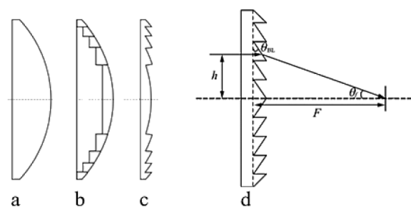
Figure 9. (a) Plano-convex lens; (b) curved Fresnel lens; (c) planar Fresnel lens; (d) planar Fresnel lens design schematic. Reprinted with permission from Ref. [27].
