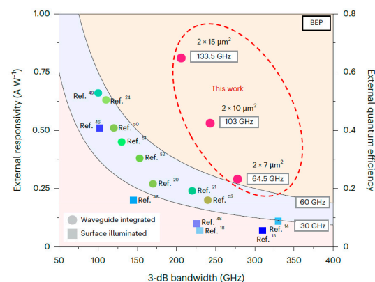
Figure 5. Performance comparison of waveguide-coupled and surface-illuminated PDs. Reprinted with permission from Ref. [22].
