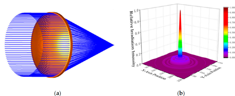
Figure 10. (a) Fresnel lens appearance and ray tracing; (b) Fresnel lens focal plane radiation intensity. Reprinted with permission from Ref. [27].
