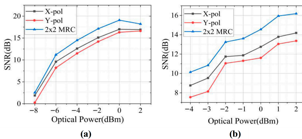
Figure 13. Input power into the PD as a function of SNR for (a) 16 GBaud and (b) 32 GBaud QPSK signals in a dual-polarization MIMO system after wireless transmission. Reprinted with permission from Ref. [28].
