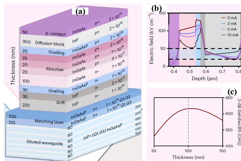
Figure 2. (a) Epitaxial layer configuration of the spot-size converter (SSC) and MUTC-PD. The epitaxial stack starts with a diluted waveguide formed by six InGaAsP layers, whose thicknesses gradually increase from 100 nm to 250 nm in 30 nm steps, separated by 80 nm InP spacer layers. Two additional InGaAsP layers positioned above the diluted waveguide function as optical index-matching layers. In the MUTC-PD region, a 165 nm p-type InGaAs absorption layer is partially depleted, leaving a 65 nm undepleted section with a step-graded doping profile ( 5 \times 10^{17} , 1 \times 10^{18} , and 2 \times 10^{18} cm -3 ) to establish a quasi-electric field that facilitates electron transport. A 300 nm p-doped InP layer on top serves as the diffusion-blocking layer, while a 250 nm lightly n-doped InP layer beneath acts as the electron drift region. InGaAsP quaternary transition layers are incorporated at the InGaAs–InP heterointerfaces to alleviate band discontinuities. (b) Simulated electric-field distributions of the 2 \times 15 \mu\text{m}^2 device under a bias voltage of -1.5 V for different photocurrent levels. (c) Calculated transit-time-limited bandwidth as a function of the depleted absorber thickness W_d . Reprinted with permission from Ref. [22].
