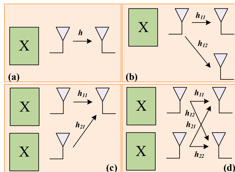
Figure 12. (a) SISO system; (b) 1 \times 2 SIMO system; (c) 2 \times 1 MISO system; and (d) 2 \times 2 MIMO system.
