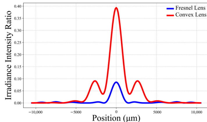
Figure 11. The relative irradiance intensity curves on the focal plane for the two types of lenses. Reprinted with permission from Ref. [27].
