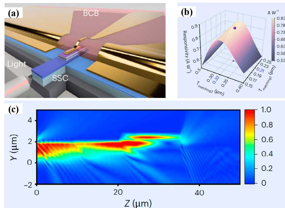
Figure 1. (a) Schematic of the device. The integrated SSC efficiently couples the incident optical signal with the active area of the MUTC-PD. The RF output signal is transmitted through a CPW taper to the contact pads of the PD. (b) Simulated external responsivity versus thickness of the first (Q1.03) and second (Q1.33) matching layers for the 2 \times 15 \mu\text{m}^2 device. (c) Simulated optical intensity as light propagates through the structure. Reprinted with permission from Ref. [22].
