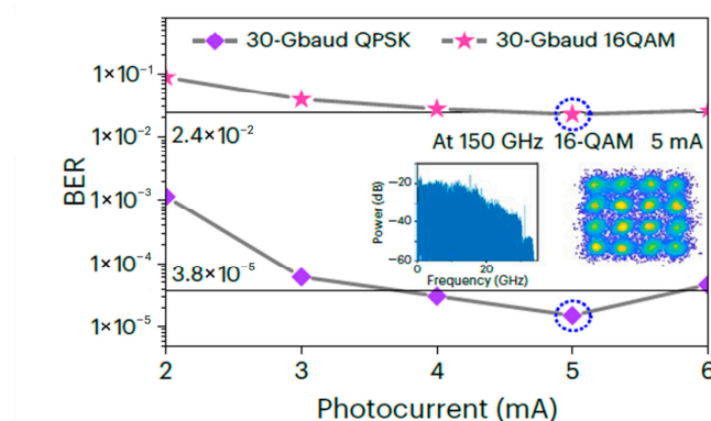
Figure 4. BER versus photocurrent for 30 Gbaud QPSK/16QAM signal at a carrier frequency of 150 GHz. Insets: electrical spectrum (left) and constellation diagram (right) for a 16QAM signal at 5 mA. Reprinted with permission from Ref. [22].
