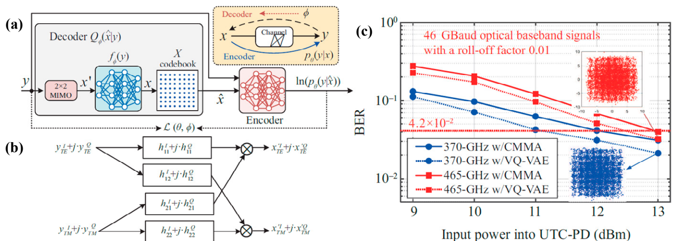
Figure 8. (a) Nonlinear compensation using VQ-VAE with (b) a classical 2 \times 2 butterfly MIMO equalizer. (c) BER vs. input power with 46 GBaud PS-64QAM with CMMA and VQ-VAE equalizers at 370 and 465 GHz. Reprinted with permission from Ref. [26].
