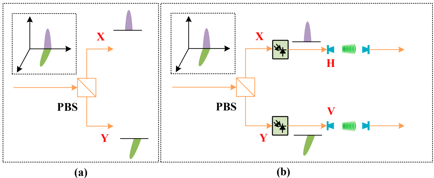
Figure 6. (a) Spectra of PDM signals after PBS with optical fiber transmission; (b) schematic diagram for polarization-multiplexing mmWave signal based on a MIMO architecture.
