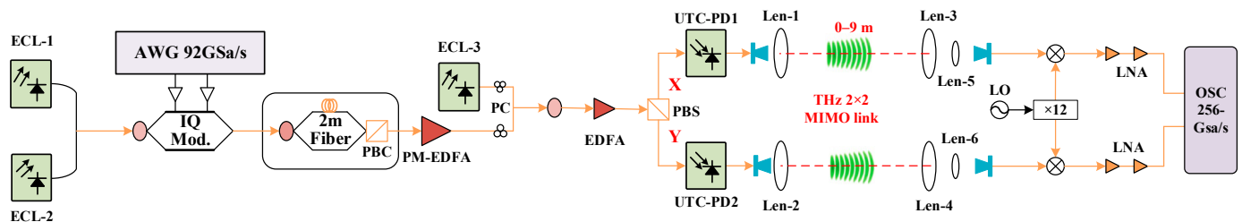
Figure 7. Experimental setup of 1 Tbps THz wireless transmission system.
