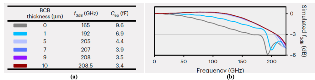
Figure 3. (a) Detailed data of the simulated 3 dB bandwidth and C_{ep} of the 2 \times 15 \mu\text{m}^2 device with varying thicknesses of BCB. (b) Simulated frequency response of the 2 \times 15 \mu\text{m}^2 device with varying thicknesses of BCB. Reprinted with permission from Ref. [22].
