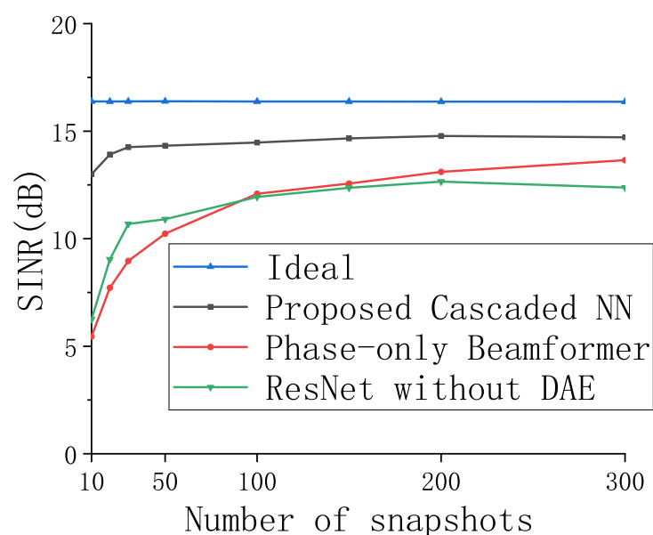
Figure 5. Output SINR versus the number of snapshots.
