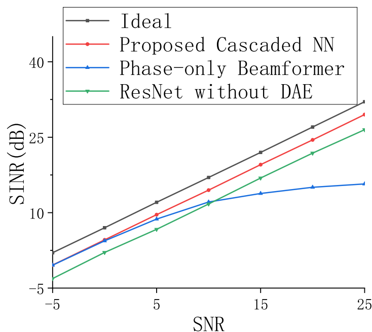
Figure 4. Output SINR versus SNR.
