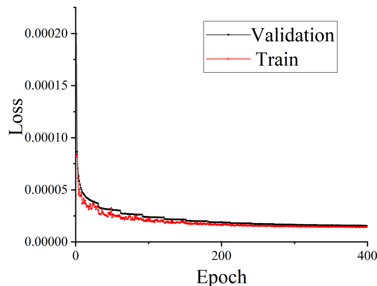
Figure 3. Training and validation loss versus epochs.
