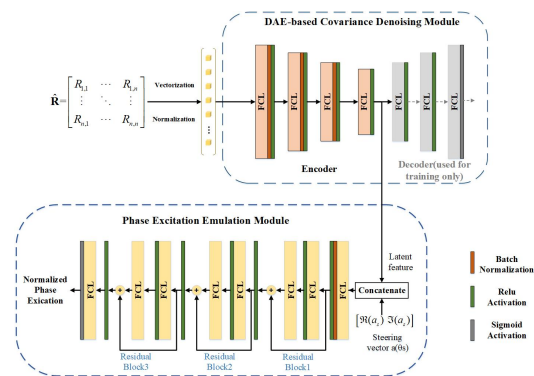
Figure 1. Cascaded neural network framework for covariance-mismatch-tolerant phase-only beamforming.
