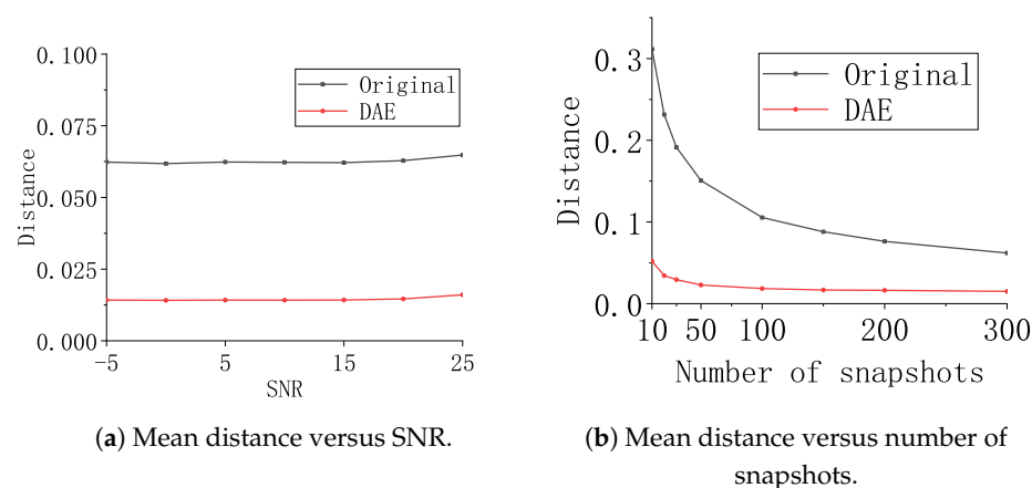
Figure 2. Reconstruction performance of the DAE.
