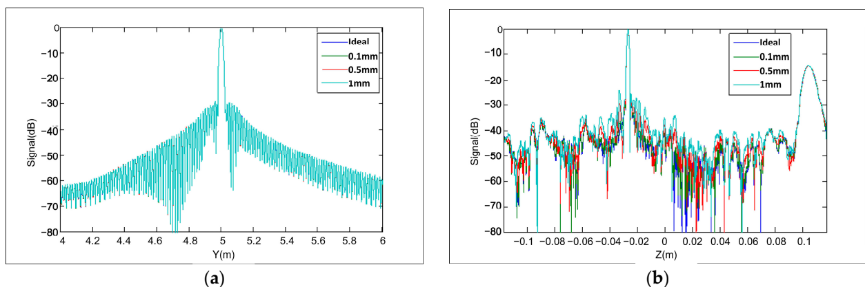
Figure 10. Imaging results with azimuth error. (a) Range imaging results; (b) elevation imaging results.
