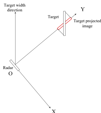
Figure 3. Imaging geometric relationship.
