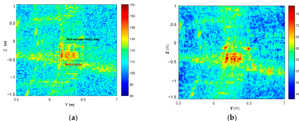
Figure 6. Metal plate imaging inside non-woven fabric. (a) Conventional processing image of the metal plate in the non-woven fabric bag; (b) range super-resolution processed image of the metal plate in the non-woven fabric bag.
