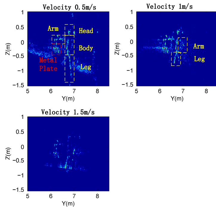
Figure 7. Imaging results of non-cooperative targets at different velocities.
