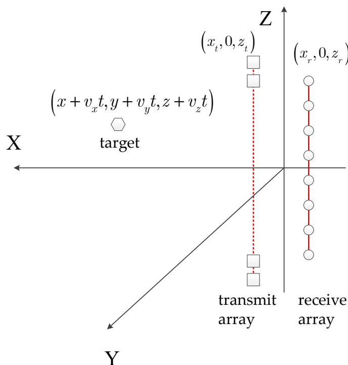
Figure 2. XOZ coordinate system array distribution model.
