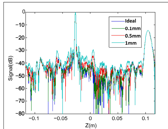
Figure 9. Elevation imaging results with elevation error.
