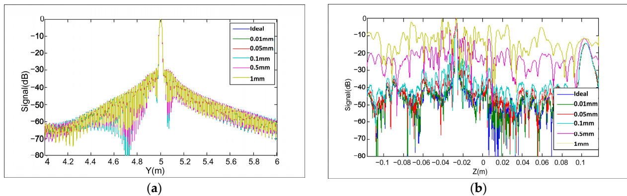
Figure 11. Imaging results. (a) Range imaging results; (b) elevation imaging results.
