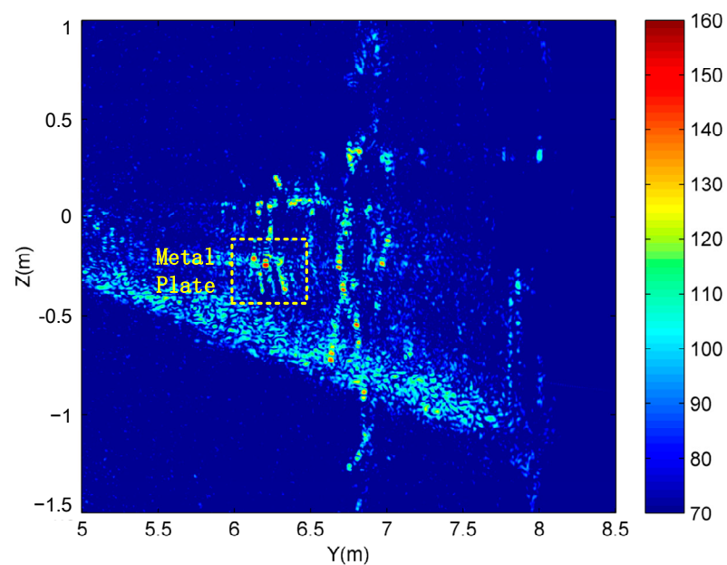
Figure 8. Imaging results of non-cooperative targets after multi-velocity fusion.
