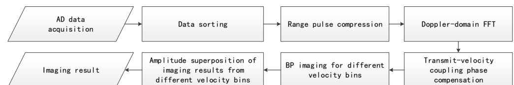
Figure 4. MIMO millimeter-wave radar imaging algorithm flow.
