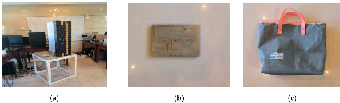
Figure 5. MIMO radar; imaging target; and obstruction. (a) MIMO radar prototype; (b) metal plate; and (c) non-woven fabric bag.
