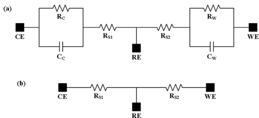
Figure 5. Equivalent impedance model (a) and simplified model (b) of the electrochemical cell, where the black squares represent the connection terminals for the electrodes.
