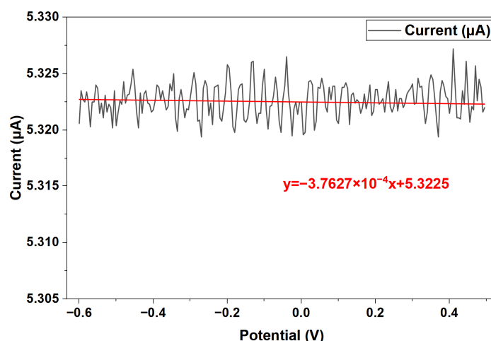
Figure 7. DPV test curve (black line) and linear fitting curve (red line) of the AFE for a 4.7 kΩ simulated electrochemical cell.
