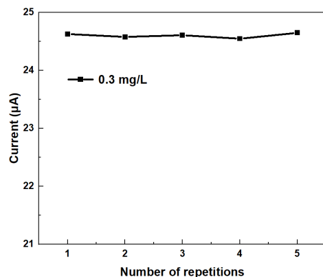
Figure 12. Repeatability of the proposed system with a solution containing 0.3 mg/L of \text{Cu}^{2+} .
