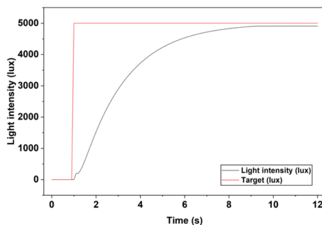
Figure 9. Step response of the incremental PID dimming algorithm.
