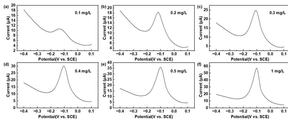
Figure 11. DPV response curves measured by the PAEcStat under different \text{Cu}^{2+} concentrations: (a) 0.1 mg/L, (b) 0.2 mg/L, (c) 0.3 mg/L, (d) 0.4 mg/L, (e) 0.5 mg/L, and (f) 1 mg/L.
