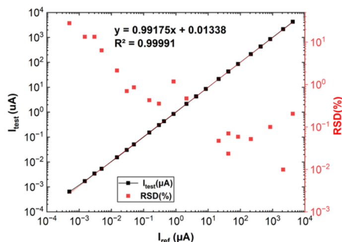
Figure 6. Measured current versus theoretical current and its relative standard deviation.
