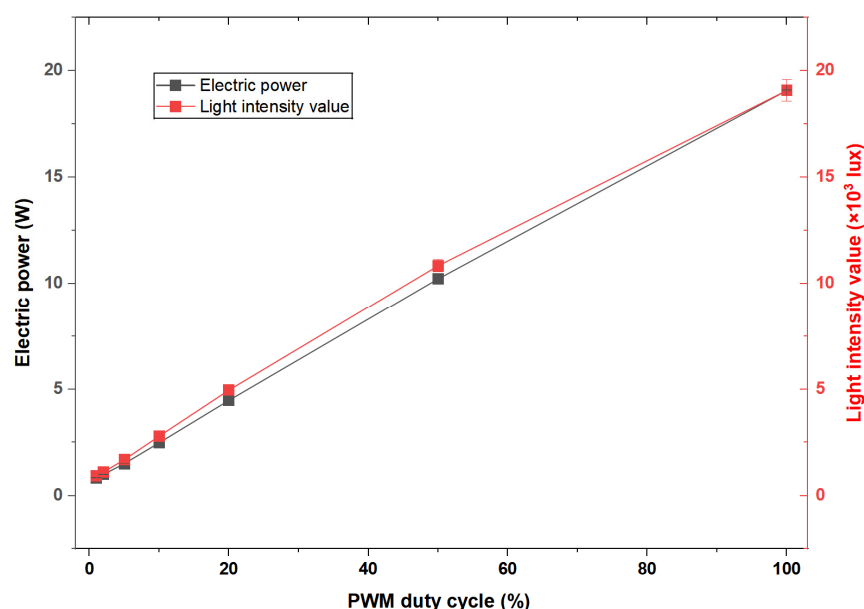
Figure 8. Input PWM duty cycle versus output electrical power and illumination intensity.
