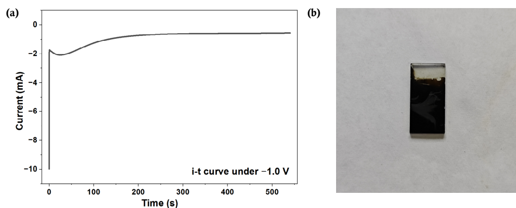
Figure 4. Potentiostatic electrodeposition i – t curve of the composite electrode at -1.0\text{ V} (a) and the fabricated \text{Co}_3\text{O}_4/\text{WO}_x/\text{FTO} electrode (b).
