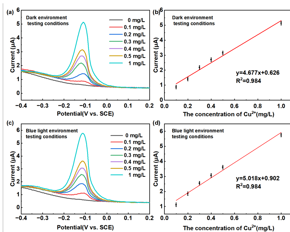
Figure 10. Validation of the electrode's photo-response. (a) DPV responses and (b) calibration curve of the \text{Co}_3\text{O}_4/\text{WO}_x/\text{FTO} electrode to different concentrations of copper ions under dark conditions; (c) DPV responses and (d) calibration curve under blue light illumination.
