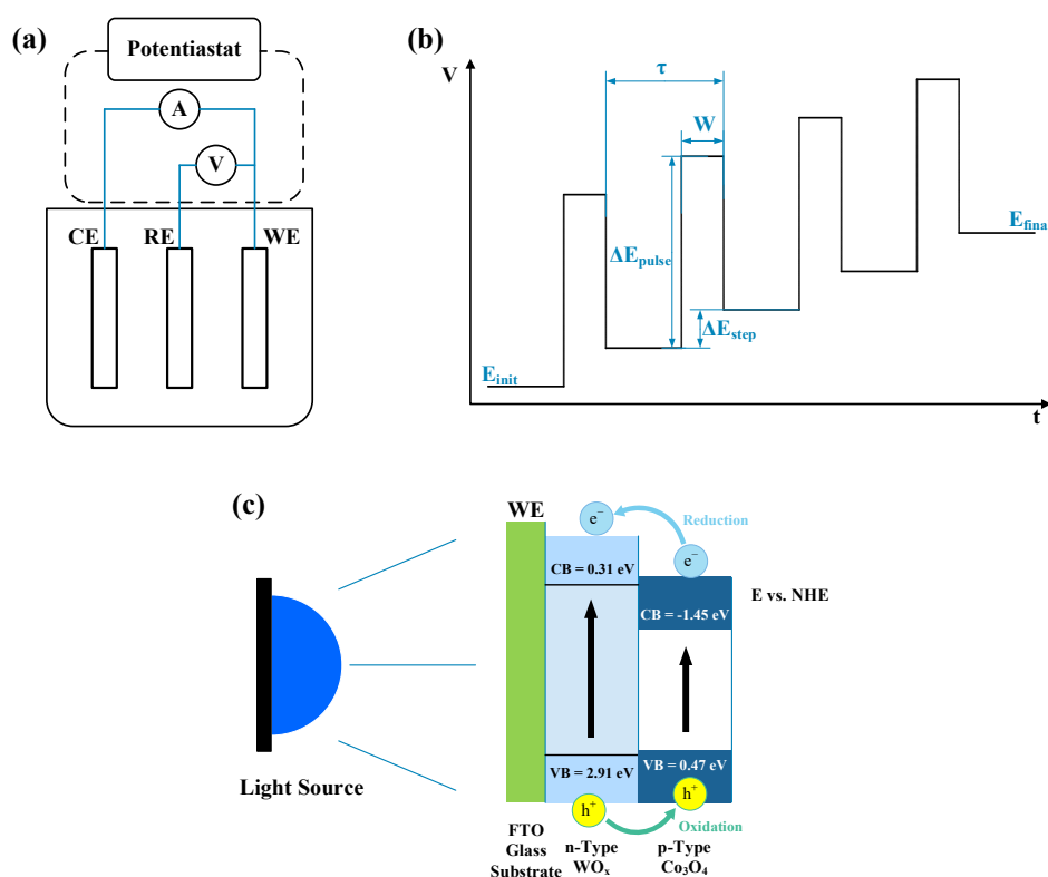
Figure 1. (a) Working principle of the three-electrode system. (b) Excitation signal waveform of DPV. (c) Principle of photo-assisted electrochemistry.
