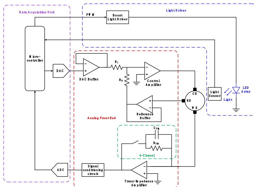
Figure 3. Schematic diagram of the overall structure of the PAEcStat, which primarily consists of a light source module and an electrochemical AFE.
