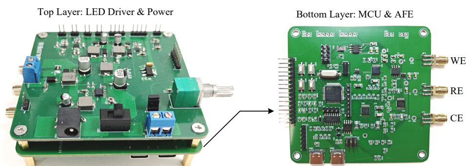
Figure 2. The designed PAEcStat system primarily comprises two parts: the electrochemical AFE and the light source driver circuit.
