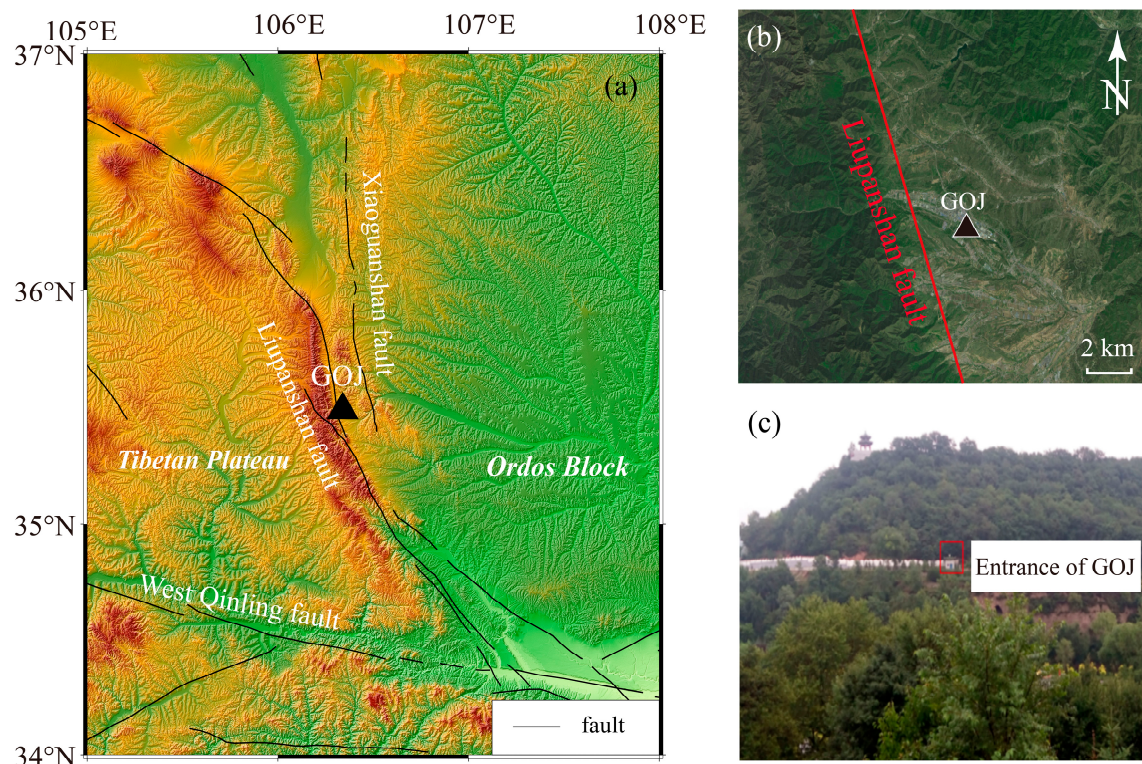
Figure 2. (a) Location of the GOJ (black triangle) and tectonic setting, (b) the surrounding mountains and fault, (c) a photo of the mountain coverage.
