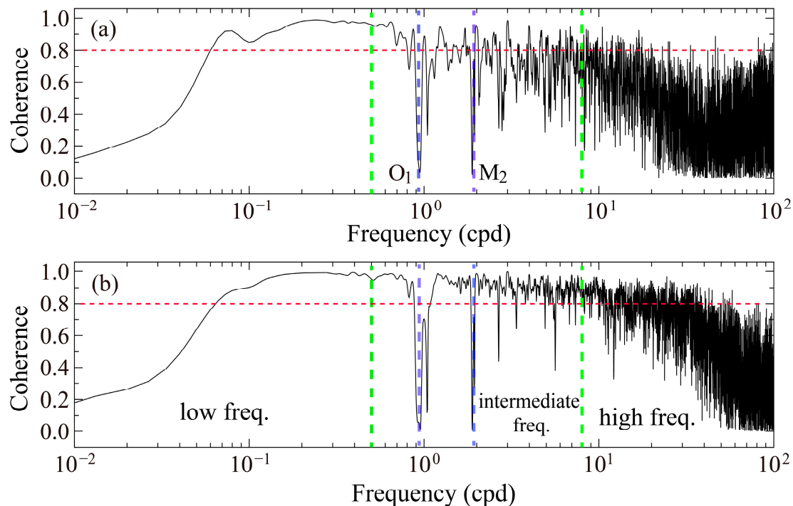
Figure 4. Coherence spectrum of NS (a) and EW (b) components for strain and pressure waves of different periods. The horizontal red dashed line means that the coherence value is equal to 0.8. The left and right vertical blue dashed lines indicate the O_1 and M_2 tidal constituents, respectively. The left and right vertical green dashed lines indicate 0.5 cpd and 8 cpd, respectively. Note that the threshold of coherence value is set as 0.8 here in order to obtain a more robust transfer function.
