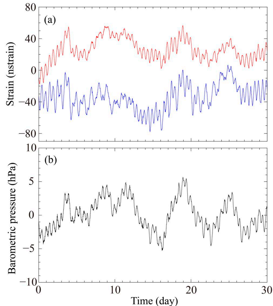
Figure 1. Variations in strain (extension negative) (a) and pressure wave (b) at the Geodynamical Observatory Jingyuan from 1 to 30 October 2023. The red and blue lines indicate the NS and EW components, respectively. Note: nstrain = 10^{-9} .
