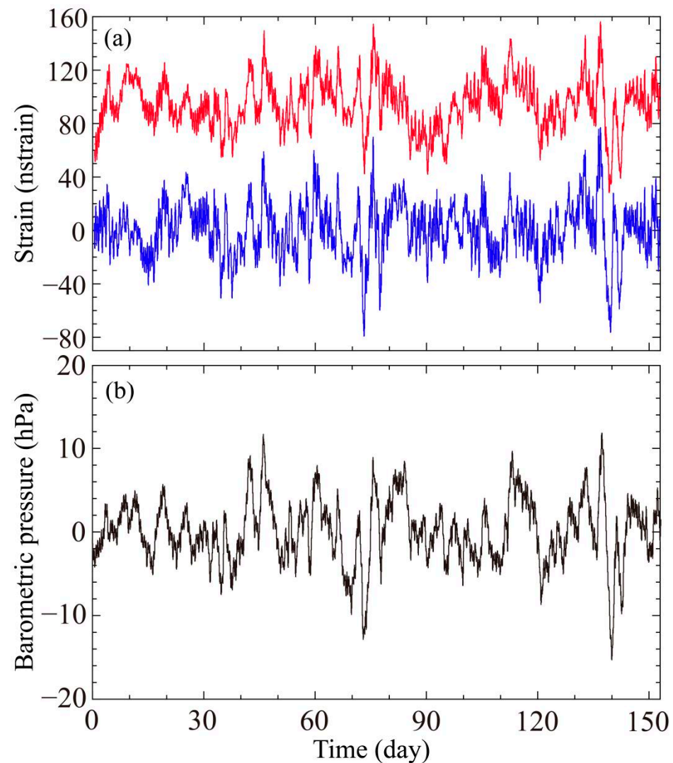
Figure 3. Time-varying curves of strains (a) and barometric pressures (b) from 1 October 2023 to 1 March 2024. The red and blue lines indicate the NS and EW components of strain, respectively.
