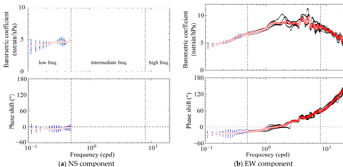
Figure 5. Transfer function (black dot) and its median value (red circle) for the response of strain to pressure waves at different frequencies. Note: a positive phase shift indicates that the strain lags behind the pressure wave, and vice versa. The left and right vertical black dashed lines indicate 0.5 cpd and 8 cpd, respectively. The horizontal black dashed line indicates zero-phase-shift. The blue vertical lines mark the 95% confidence intervals.
