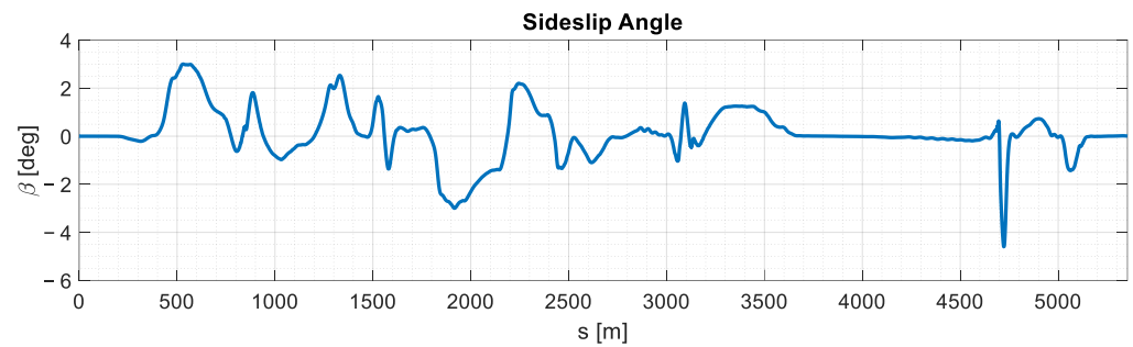
Figure 19. Vehicle yaw-rate and sideslip-angle responses for the representative K_r = 0.5 case.
