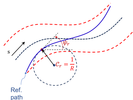
Figure 2. Geometric interpretation of the reference path. The blue solid curve represents the reference path, the red dashed curves denote the track boundaries, the black arrow indicates the path direction, \psi_r is the reference heading angle, and \mathcal{C}_r = \frac{1}{R} is the local path curvature.
