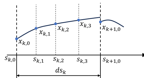
Figure 10. The direct collocation with q = 3 in a segment ds_k .
