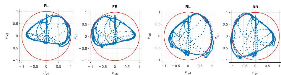
Figure 16. Normalized tire working points for the K_r = 0.5 case. The blue markers represent the normalized tire operating points during the simulation, while the red circle denotes the normalized tire–road adhesion limit.
