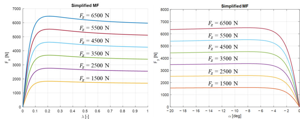
Figure 8. Steady-state Magic Formula tire characteristics. The side-slip angle is shown with its signed value according to the vehicle-model convention; the negative sign indicates the assumed tire side-slip direction.
