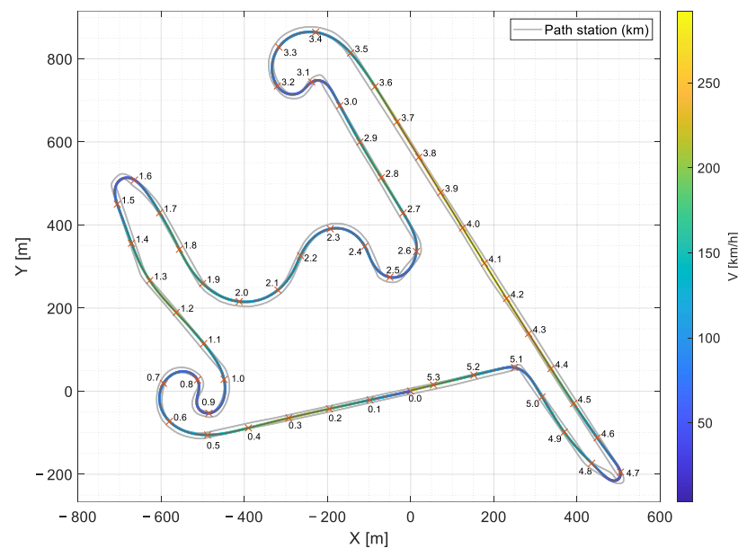
Figure 13. Representative NMPC path-tracking result for K_r = 0.5 .
