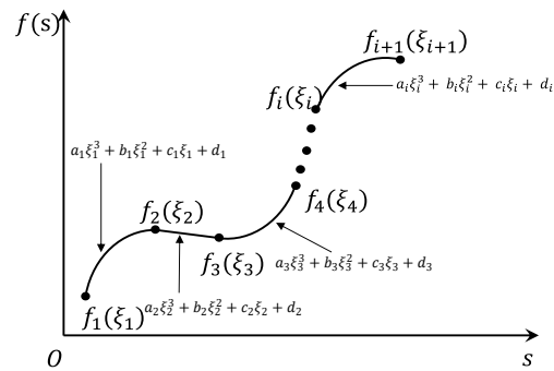
Figure 1. Cubic spline interpolation using the local coordinate \xi_i = s - s_i for each spline segment.
