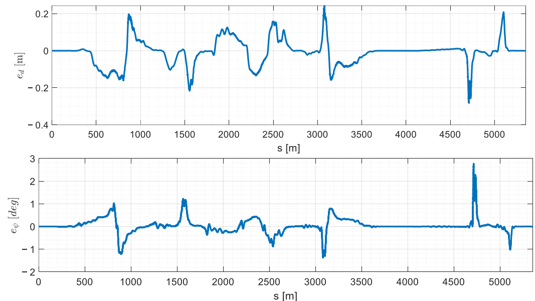
Figure 14. Representative path-tracking errors for K_r = 0.5 .
