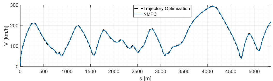
Figure 18. Velocity-tracking response for the representative K_r = 0.5 case. The black dashed line represents the TRO-optimized velocity profile, while the blue solid line denotes the NMPC tracking response.
