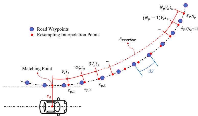
Figure 11. Preview path-station update scheme for NMPC reference generation. The black and red dashed curves denote the reference path and preview sequence, while the blue and red markers represent the road waypoints and resampled points, respectively.
