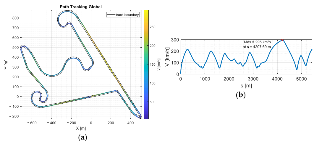
Figure 12. Representative TRO optimization result for K_r = 0.5 . (a) Optimized global trajectory with velocity indicated by the color bar and track boundaries shown in black; (b) Optimized velocity profile along the curvilinear coordinate s .
