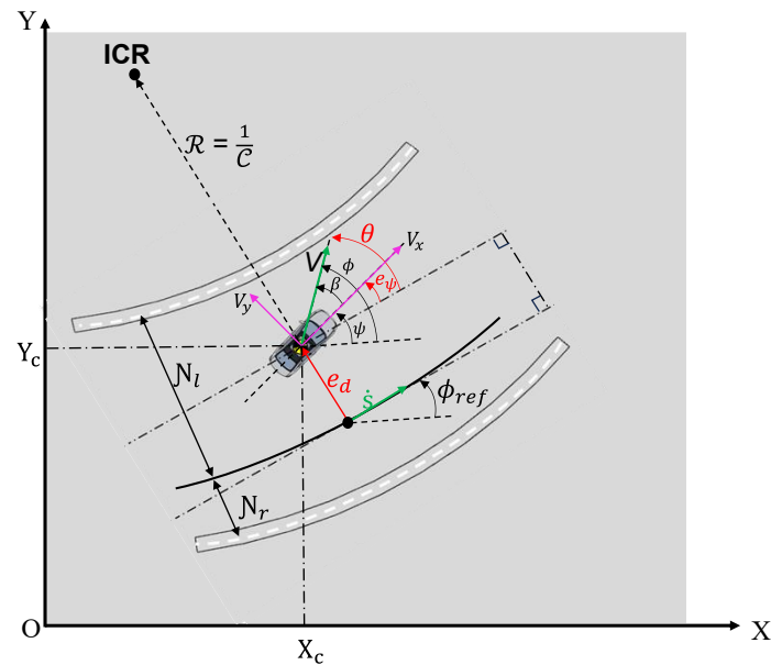
Figure 5. Relationship between the vehicle and the reference path kinematics. The black curve represents the reference path, the gray curves denote the track boundaries, the green arrows indicate the reference direction, and the red arrows represent the vehicle states and tracking errors.
