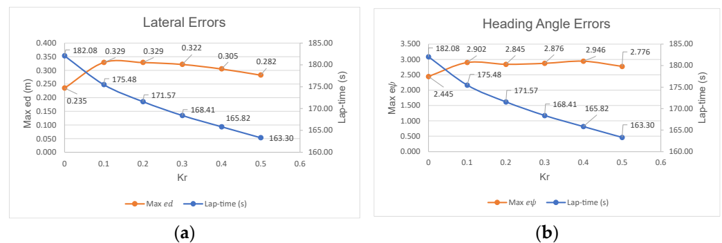
Figure 15. Comparison of maximum tracking errors and lap time under different torque distribution gains. (a) Maximum lateral deviation and corresponding lap time; (b) Maximum heading-angle error and corresponding lap time.
