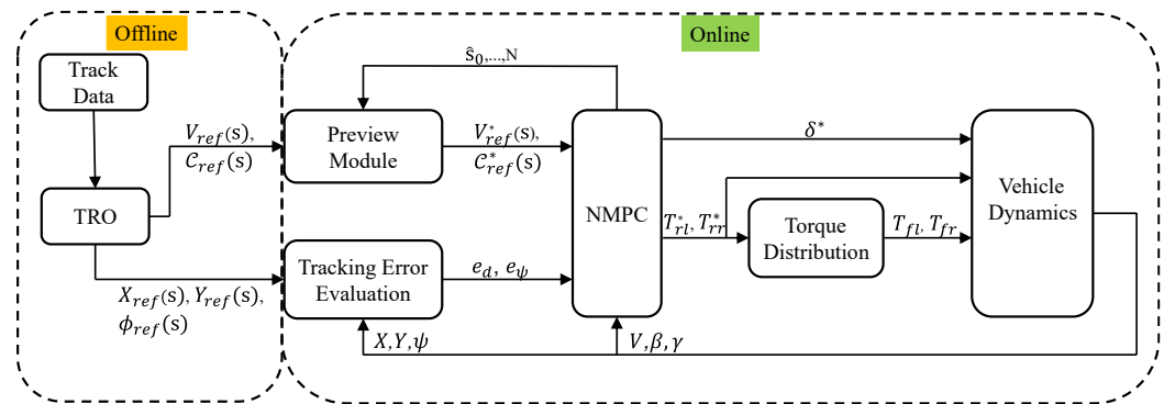
Figure 9. Overall offline–online control framework integrating TRO, NMPC, and virtual 4WD torque distribution. The yellow region represents the offline trajectory optimization process, while the green region represents the online control process.
