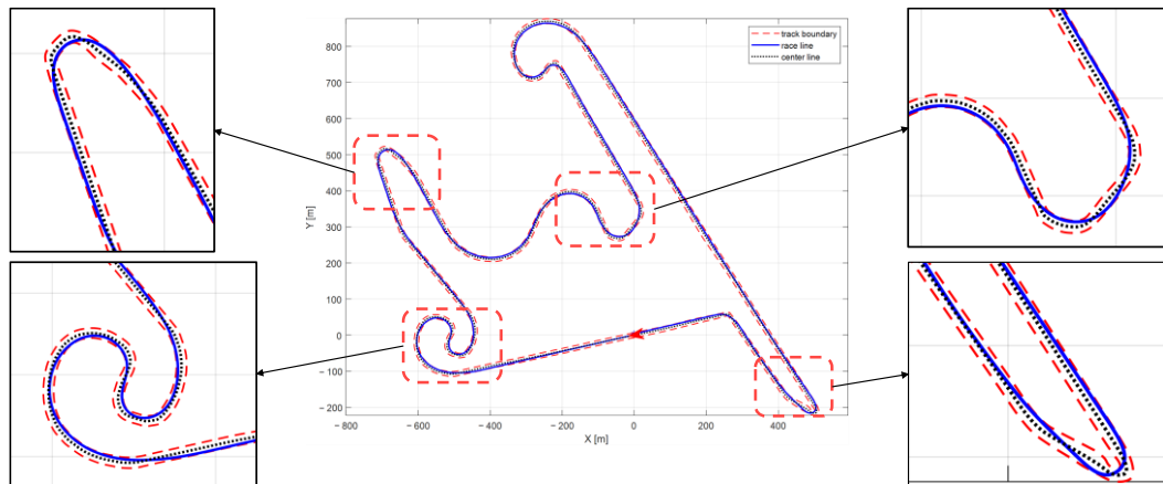
Figure 3. Geometric representation of the reference path and track boundaries. The blue solid line denotes the spline-fitted path, the black dashed line represents the original centerline, and the red dashed lines indicate the track boundaries.
