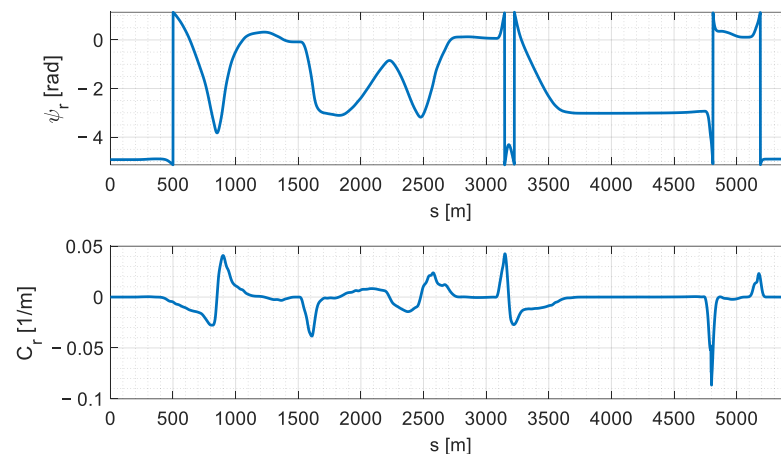
Figure 4. Reference heading angle and path curvature.
