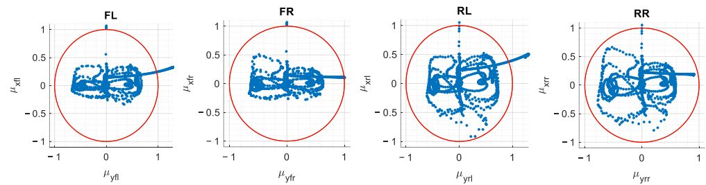
Figure 17. Normalized tire working points for the K_r = 0.6 case. The blue markers represent the normalized tire operating points during the simulation, while the red circle denotes the normalized tire–road adhesion limit.
