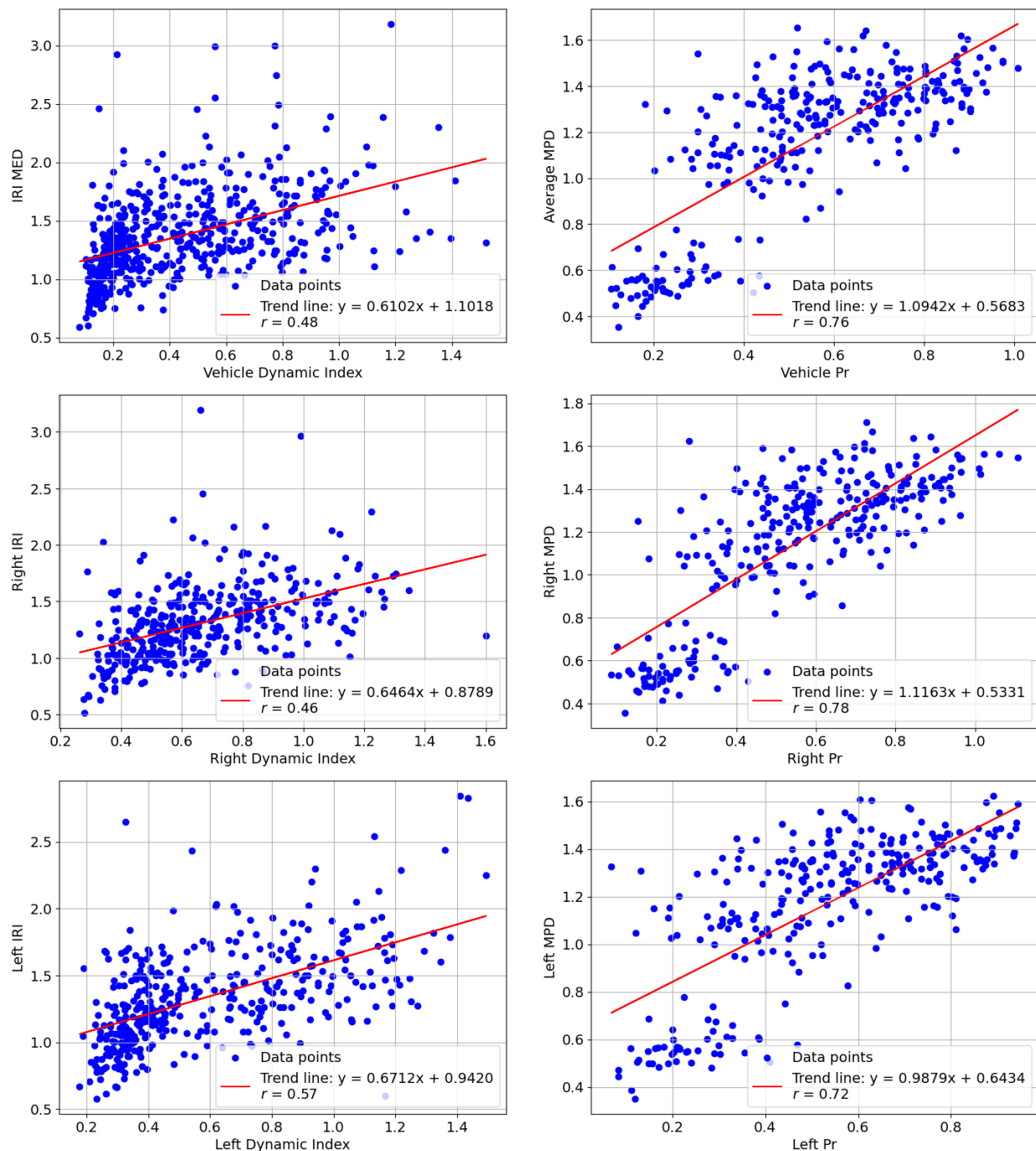
Figure 1. Correlations between smart tire and ARAN indicators (sectioning method A).
