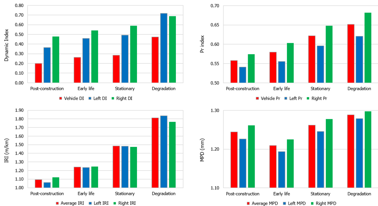
Figure 4. Time-dependent trends of smart tire and ARAN indicators (open-graded wearing courses).
