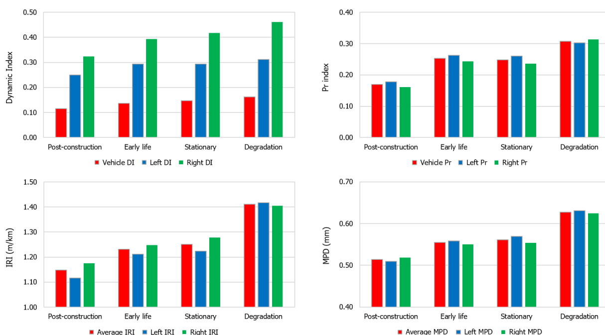
Figure 3. Time-dependent trends of smart tire and ARAN indicators (dense-graded wearing courses).
