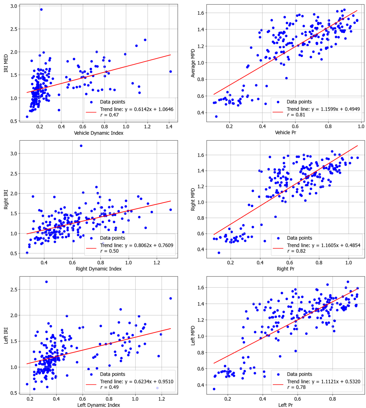
Figure 2. Correlations between smart tire and ARAN indicators (sectioning method B).
