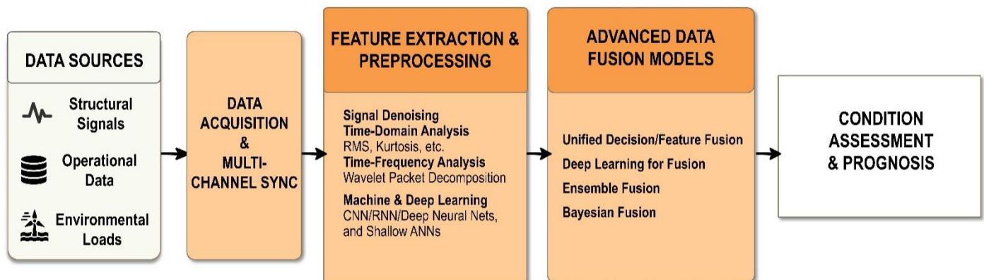
Figure 3. A generalized multi-source data fusion framework for condition assessment and prognosis.
