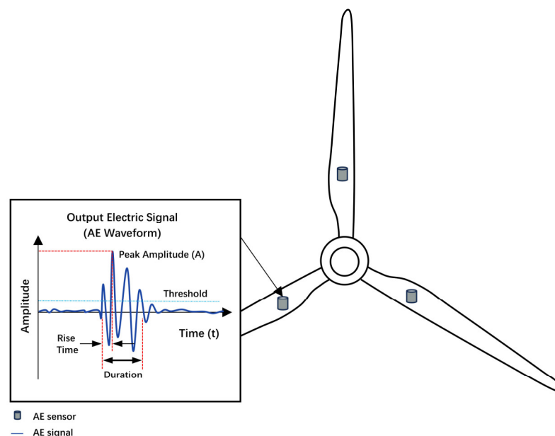
Figure 1. Schematic diagram of acoustic emission (AE) signal feature extraction.
