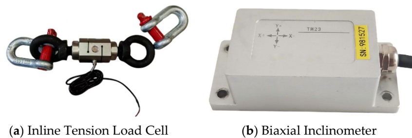
Figure 2. Sensors for floating offshore wind turbine (FOWT) mooring system monitoring.
