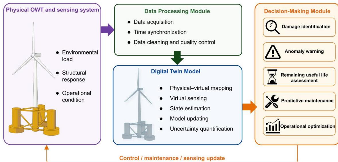
Figure 5. Schematic framework of digital twin (DT)-based structural health monitoring (SHM) for offshore wind turbines (OWTs).
