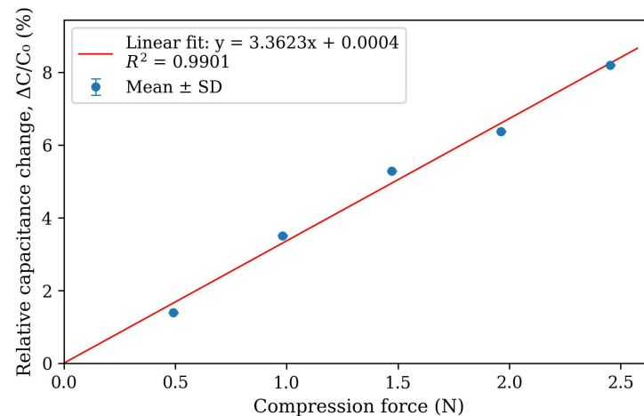
Figure 5. Linear correlation between compression force on the capacitive sensor and the relative change, \Delta C/C_0 (%), in the sensor capacitance. Markers indicate the mean values at each force level, error bars represent the standard deviation of the recorded samples, and the red line represents the linear regression fitted to the mean values. Error bars are smaller than the marker size because the standard deviation of the 1000 samples at each force level was small.
