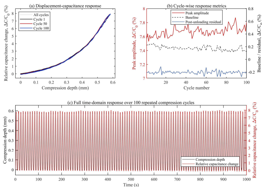
Figure 7. Low-frequency repeated-compression response of the capacitive sensor over 100 cycles. (a) Superimposed displacement–capacitance responses over 100 cycles, with Cycles 1, 50, and 100 highlighted. (b) Cycle-wise peak amplitude, baseline, and post-unloading residual response. (c) Full time-domain response of compression depth and relative capacitance change over 100 repeated compression cycles.
