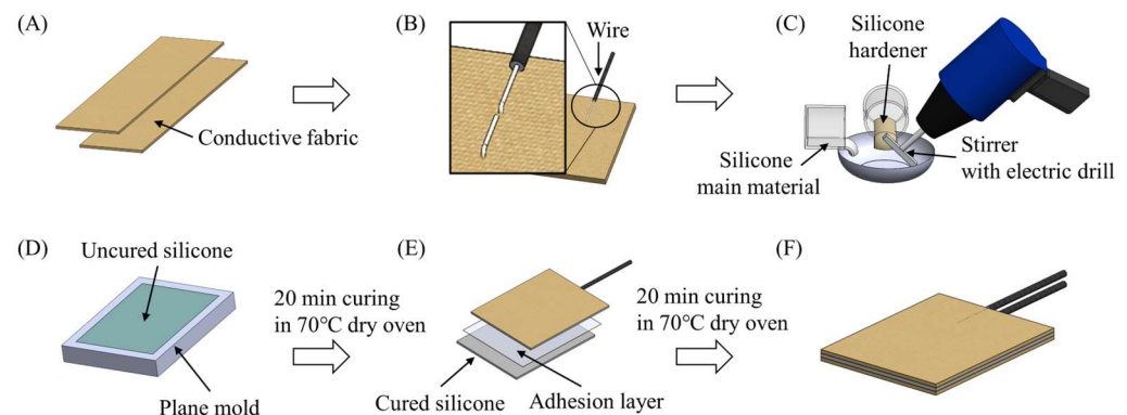
Figure 3. Fabrication process of the capacitive sensors using conductive fabrics and silicone rubber.
