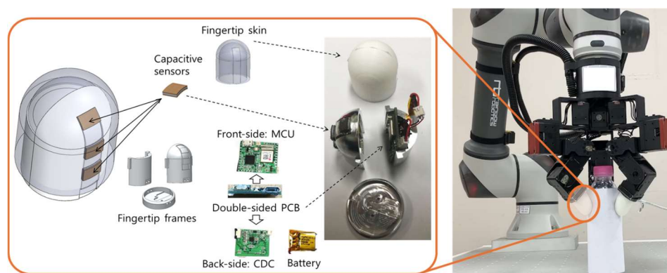
Figure 8. Parts and assembly of the developed module.
