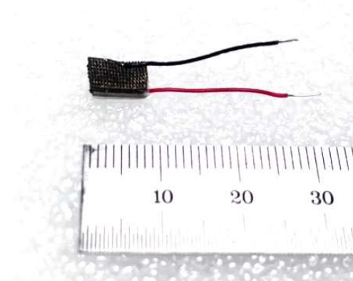
Figure 4. Fabricated capacitive sensor.
