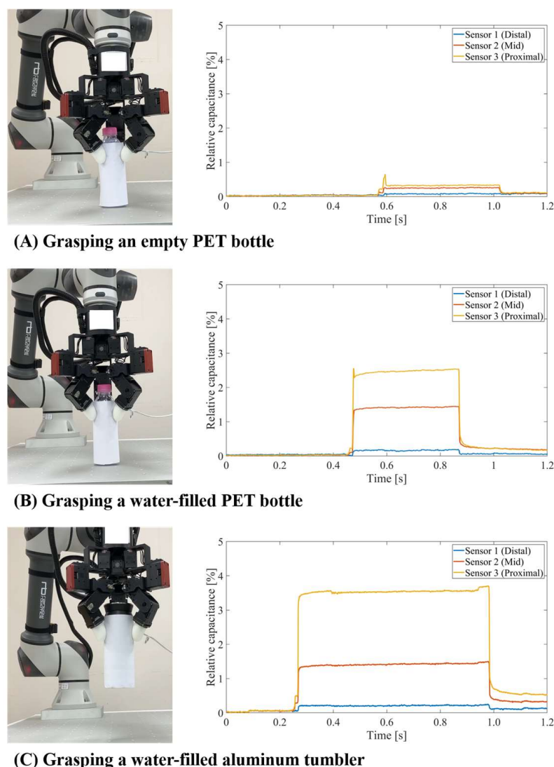
Figure 9. Relative capacitance responses during robotic grasping of three cylindrical objects: (A) empty PET bottle, (B) water-filled PET bottle, and (C) water-filled aluminum tumbler. Sensor 1, Sensor 2, and Sensor 3 correspond to the distal-, mid-, and proximal-position sensors, respectively. The responses are shown as relative capacitance changes, \Delta C/C_0 (%).
