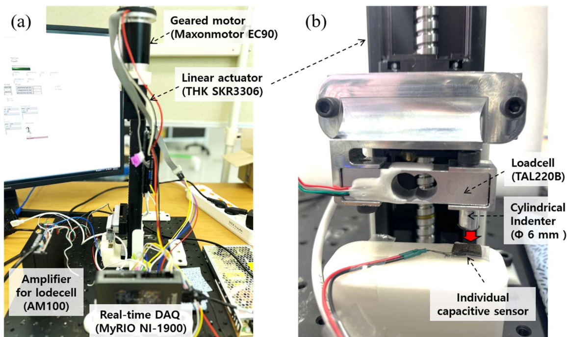
Figure 6. Experimental setup for normal compression testing of the individual capacitive sensor. (a) Custom linear actuator system consisting of a brushless DC motor, linear stage, and single-axis load cell. (b) Enlarged view of the cylindrical indenter aligned with the active sensing area of the capacitive sensor. The red arrow indicates the normal compression direction.
