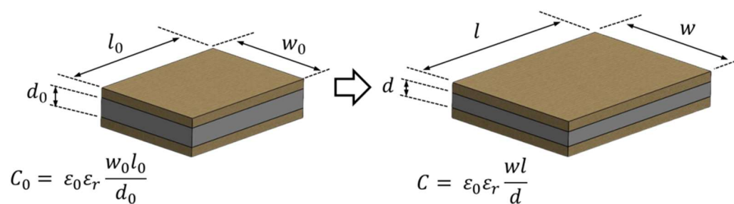
Figure 2. Basic principle of a capacitive sensor: C denotes capacitance; w and l denote the width and length of the conductive parallel plates, respectively; d denotes the thickness of the dielectric layer; \epsilon_0 and \epsilon_r denote the vacuum permittivity and relative permittivity of silicone rubber, respectively; and subscript 0 indicates the initial state.
