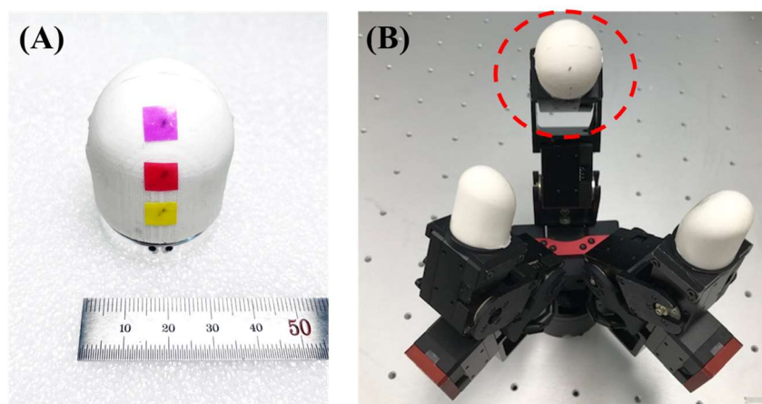
Figure 1. (A) Developed standalone tactile sensing module: the tri-color markers indicate the approximate positions of the three capacitive sensors embedded beneath the silicone fingertip skin. (B) Standalone tactile sensing module mounted on a three-fingered robotic hand: the module was installed on the tip of one finger (in red dashed circle).
