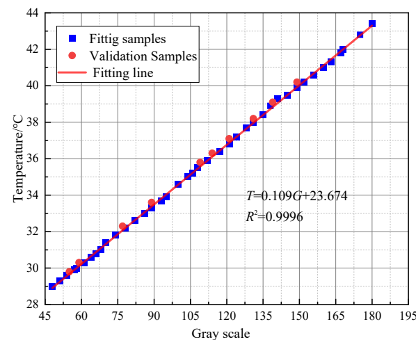
Figure 11. Linear regression between grayscale value and temperature.
