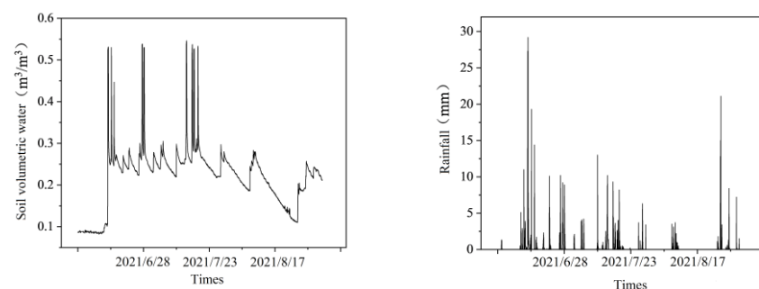
Figure 2. Meteorological and soil data.
