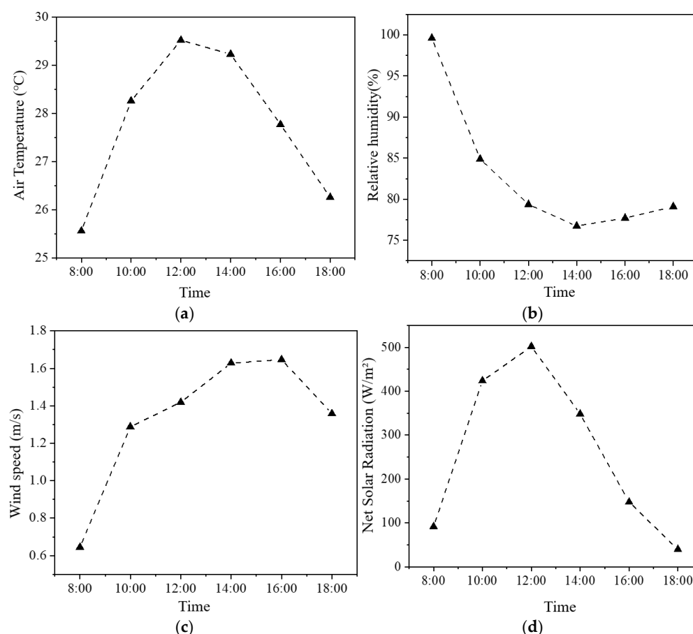
Figure 12. Related meteorological data. (a) Air temperature. (b) Relative humidity. (c) Wind speed. (d) Net Solar Radiation.
