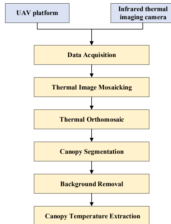
Figure 5. Workflow of the thermal infrared image processing framework for canopy temperature extraction.
