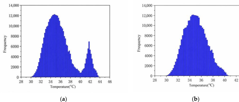
Figure 10. Histogram of infrared thermal image temperature: (a) Temperature histogram before removing soil background; (b) Temperature histogram after removing soil background.
