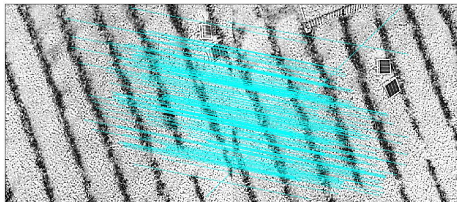
Figure 6. Feature matching results between overlapping UAV thermal images based on the SURF algorithm. The cyan lines indicate matched feature pairs between the overlapping thermal images.
