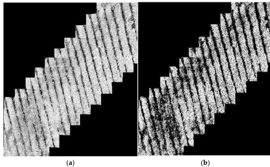
Figure 9. Image processing results: (a) Infrared thermal imaging mosaic; (b) Soil Background Removal Map.
