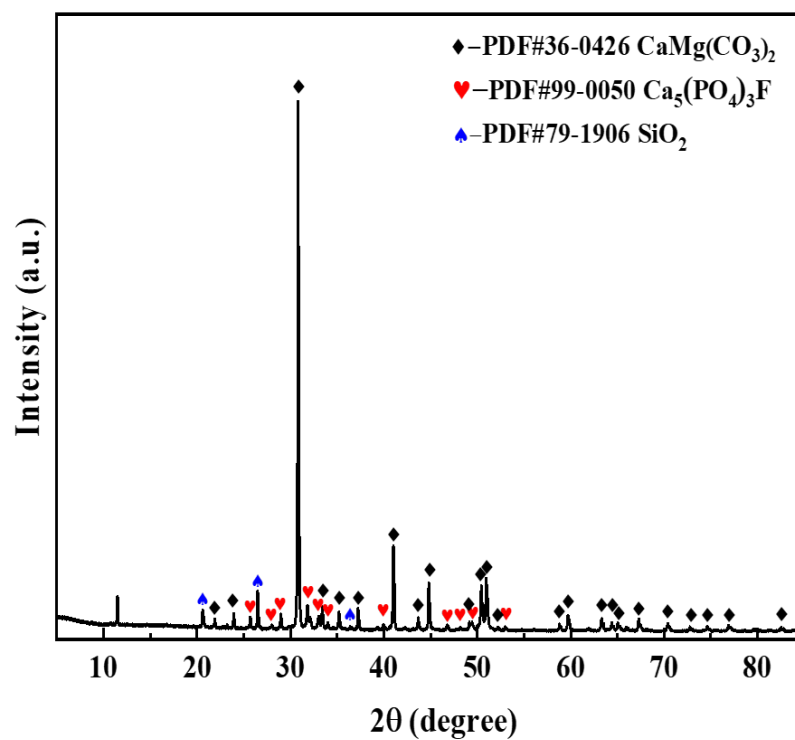
Figure 1. XRD pattern of Phosphate tailings (PTs).
