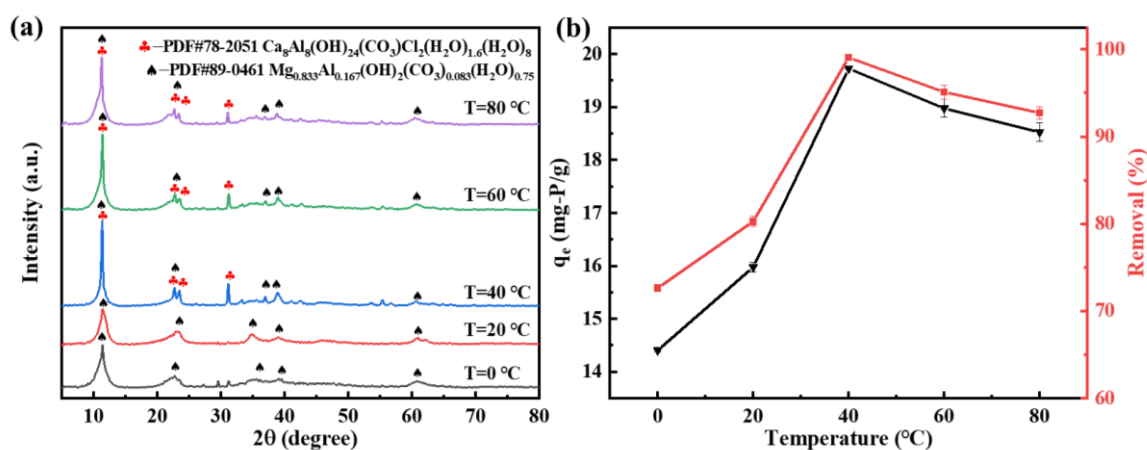
Figure 6. (a) XRD patterns and (b) phosphate removal performance of LDH samples synthesized at different aging temperatures.
