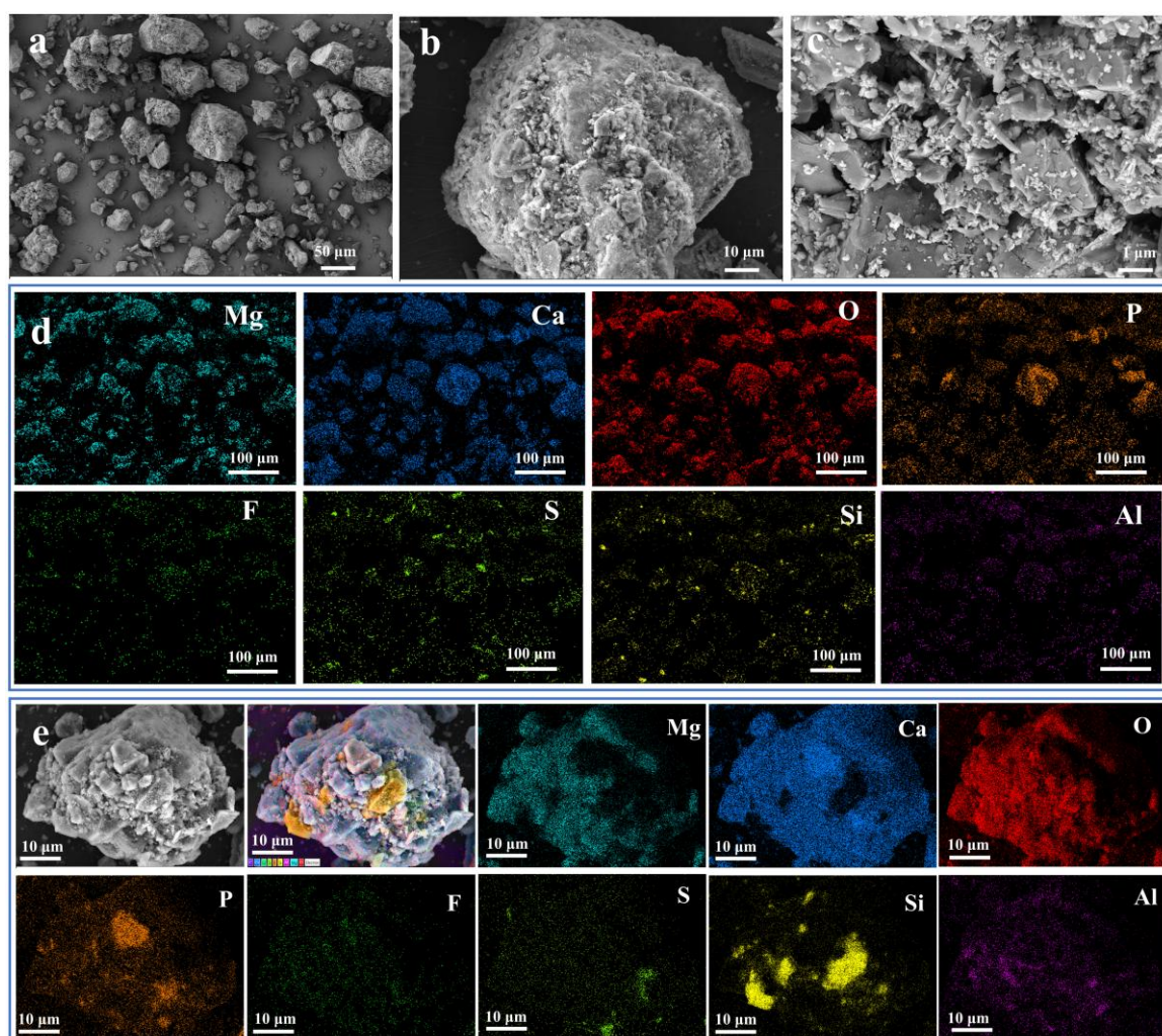
Figure 2. SEM (a–c) and EDS (d,e) analysis of PTs.
