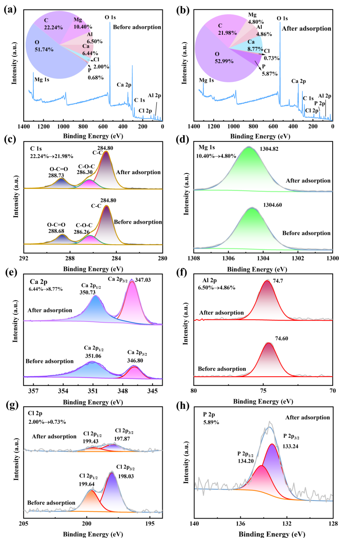
Figure 10. XPS analysis of Ca-Mg-Al LDHs before and after phosphate adsorption: (a,b) XPS survey spectra and surface elemental compositions before and after adsorption; high-resolution spectra of (c) C 1s, (d) Mg 1s, (e) Ca 2p, (f) Al 2p, (g) Cl 2p, and (h) P 2p.
