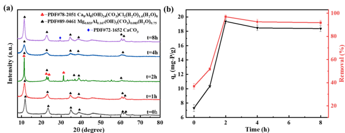
Figure 7. (a) The XRD patterns and (b) phosphate removal performance of LDH samples as a function of aging time.
