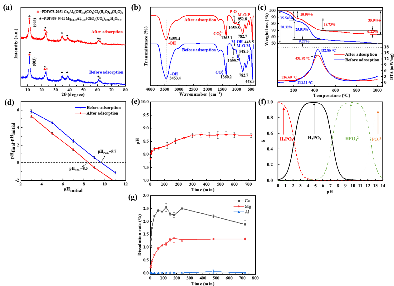
Figure 9. (a) XRD patterns, (b) FTIR spectra, (c) TG-DTA profiles, and (d) \text{pH}_{\text{PZC}} curves of LDHs before and after phosphate adsorption; (e) variation in solution pH, (f) phosphate species distribution as a function of pH during phosphate removal by Ca-Mg-Al LDHs; (g) temporal changes in the dissolution rates of major metal ions.
