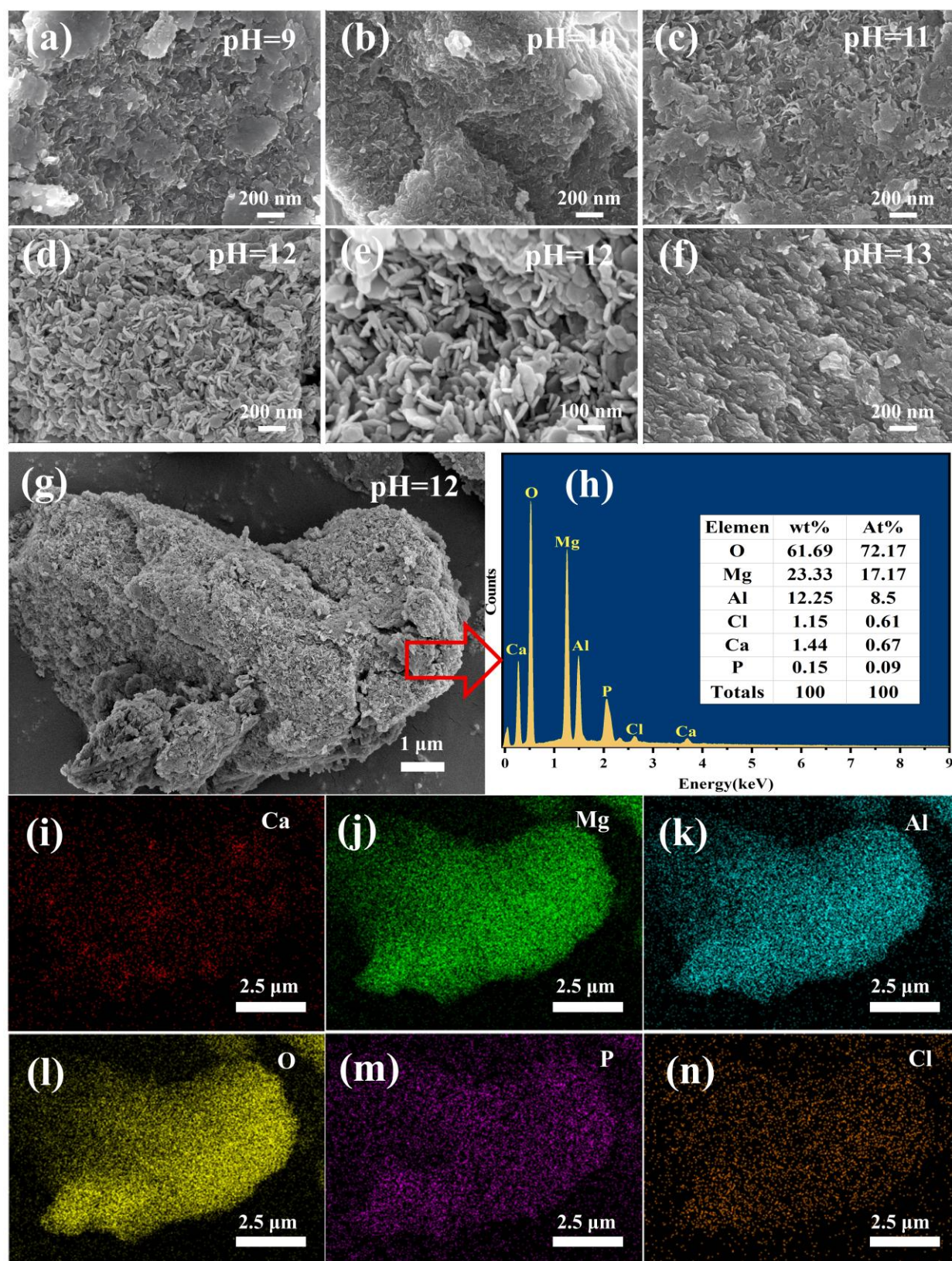
Figure 5. (a–f) SEM images of the samples prepared at pH 9–13, with panel (e) showing a higher-magnification image of the sample prepared at pH 12; (g–n) SEM-EDS results and elemental mappings of the sample prepared at pH 12, where (g) is the SEM image, (h) is the EDS spectrum, and (i–n) represent the mappings of Ca, Mg, Al, O, P, and Cl, respectively.
