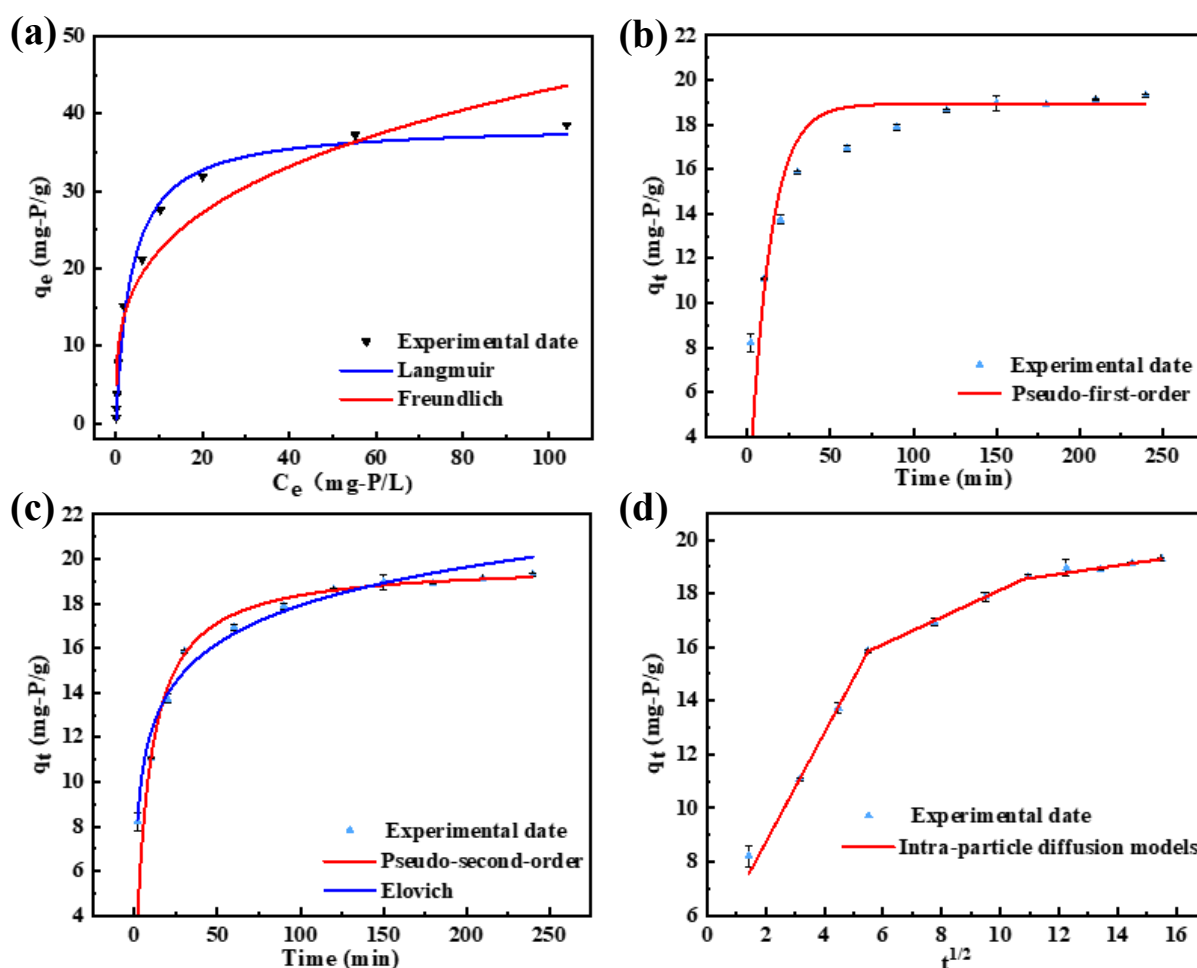
Figure 8. (a) Phosphate adsorption isotherms fitted by the Langmuir and Freundlich models; (b–d) adsorption kinetics fitted by the (b) pseudo-first-order, (c) pseudo-second-order, and (d) intraparticle diffusion models for phosphate removal by Ca-Mg-Al LDHs.
