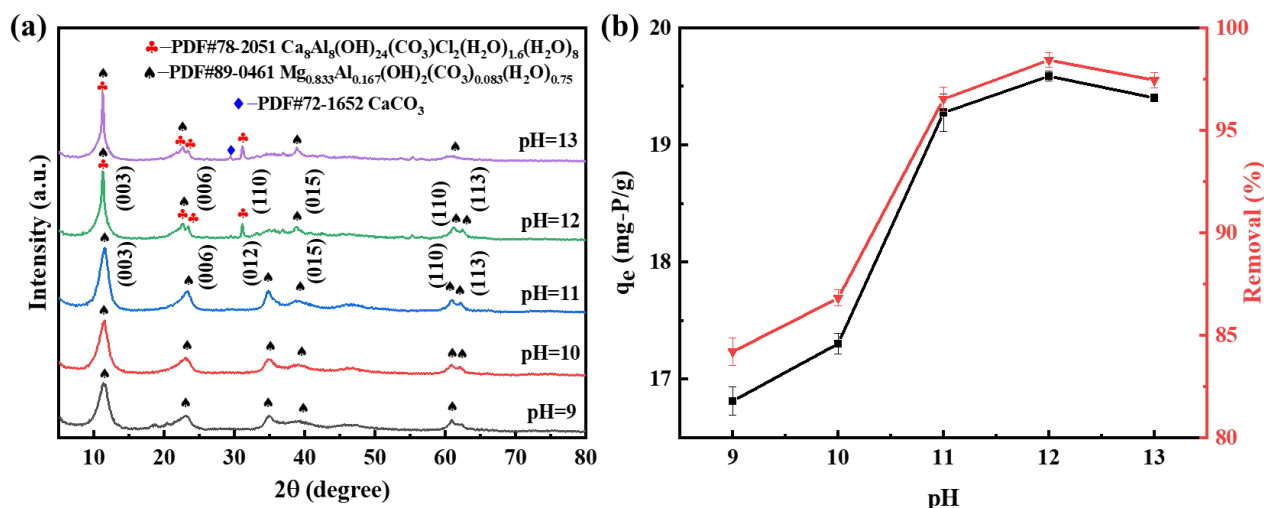
Figure 4. (a) XRD patterns and (b) phosphate removal efficiency of Ca-Mg-Al LDHs synthesized at different pH values.
