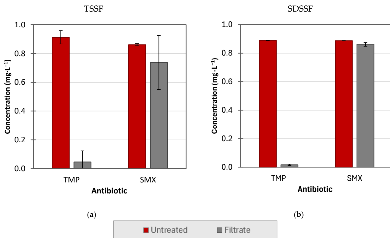
Figure 6. Graphical representation of antibiotic removal in the (a) TSSF and (b) SDSSF.
