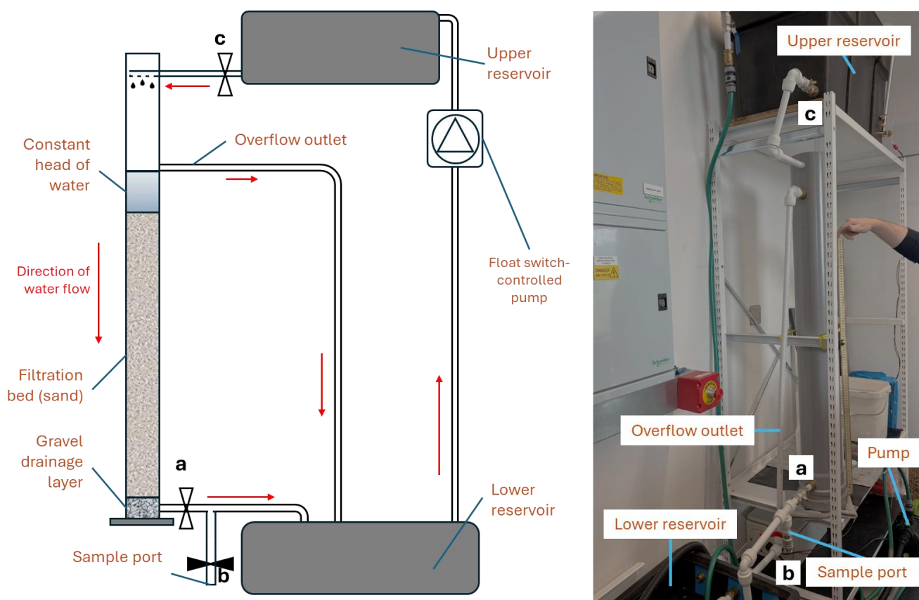
Figure 1. A schematic diagram of the slow sand filter and its recirculating arrangement (left), and a digital photograph showing the slow sand filter set-up in operation with a 1 m ruler for scale (right) (a: outlet valve which controls filtration rate; b: filtrate sample port; c: upper reservoir valve which controls overflow flow rate; red arrows indicate direction of water flow).
