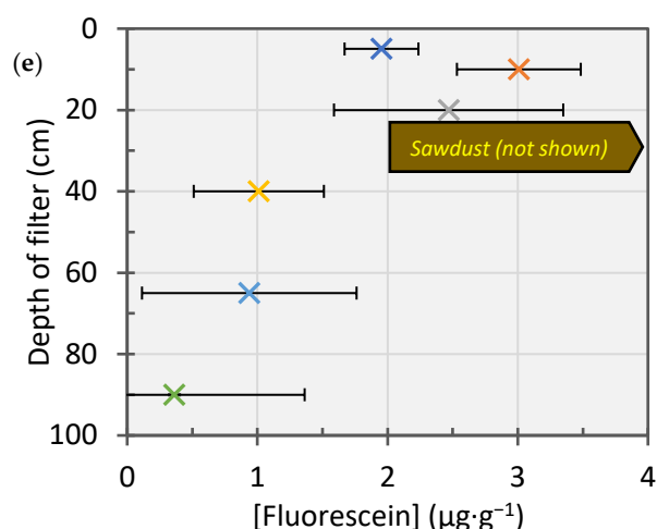
Figure 7. The enzymatic activity throughout the depth of each SSF, where (a,b) show the mean enzyme activity for each section tested for the TSSF; and (c–e) show the mean enzyme activity for each section tested for the SDSSF. ‘X’ markers show mean value. Note: Graph (c) includes all quantified depths, including the sawdust, which extended the x-axis; therefore, graph (e) is a magnified view excluding the sawdust marker to improve resolution of the data at lower concentrations.
