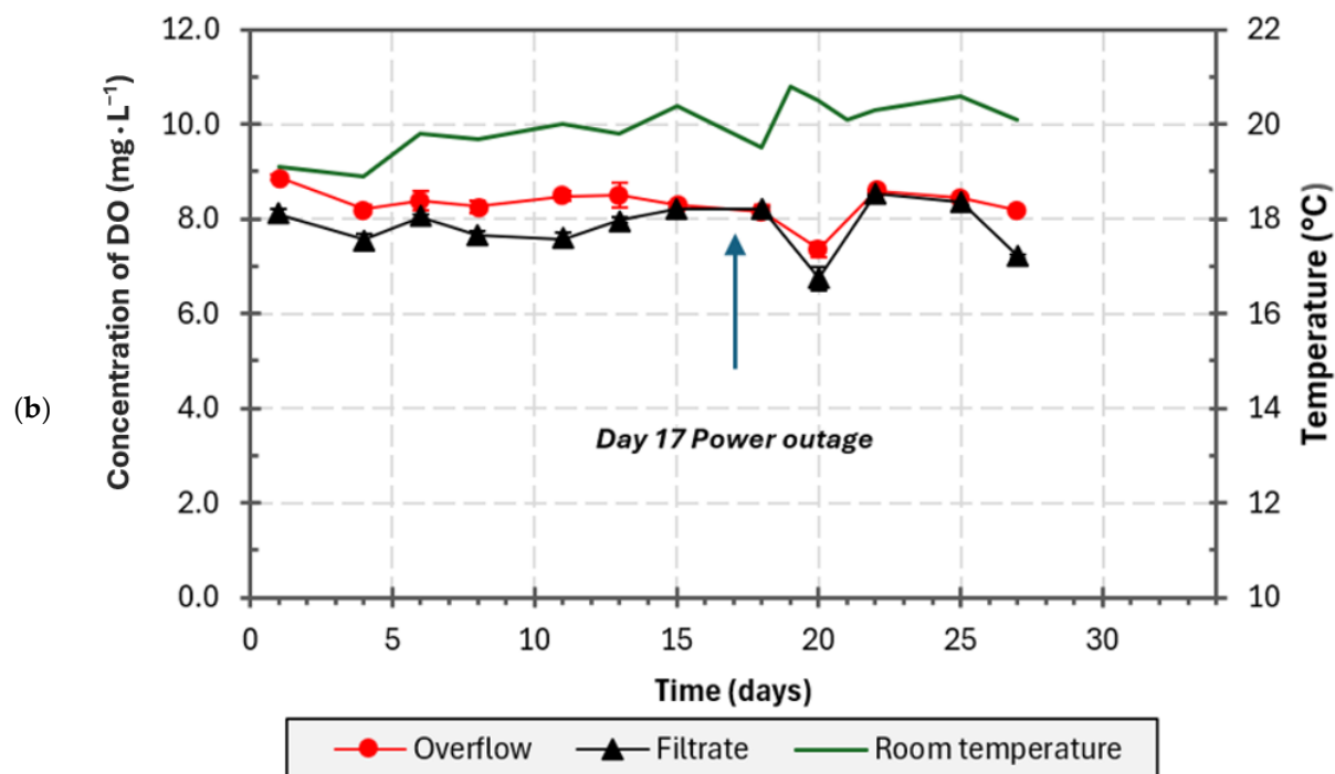
Figure 2. Concentration of dissolved oxygen in overflow and filtrate, and room temperature for the (a) TSSF and (b) SDSSF. The blue arrow represents the pump failure event outlined in the opening of Section 3.2 (SDSSF only).
