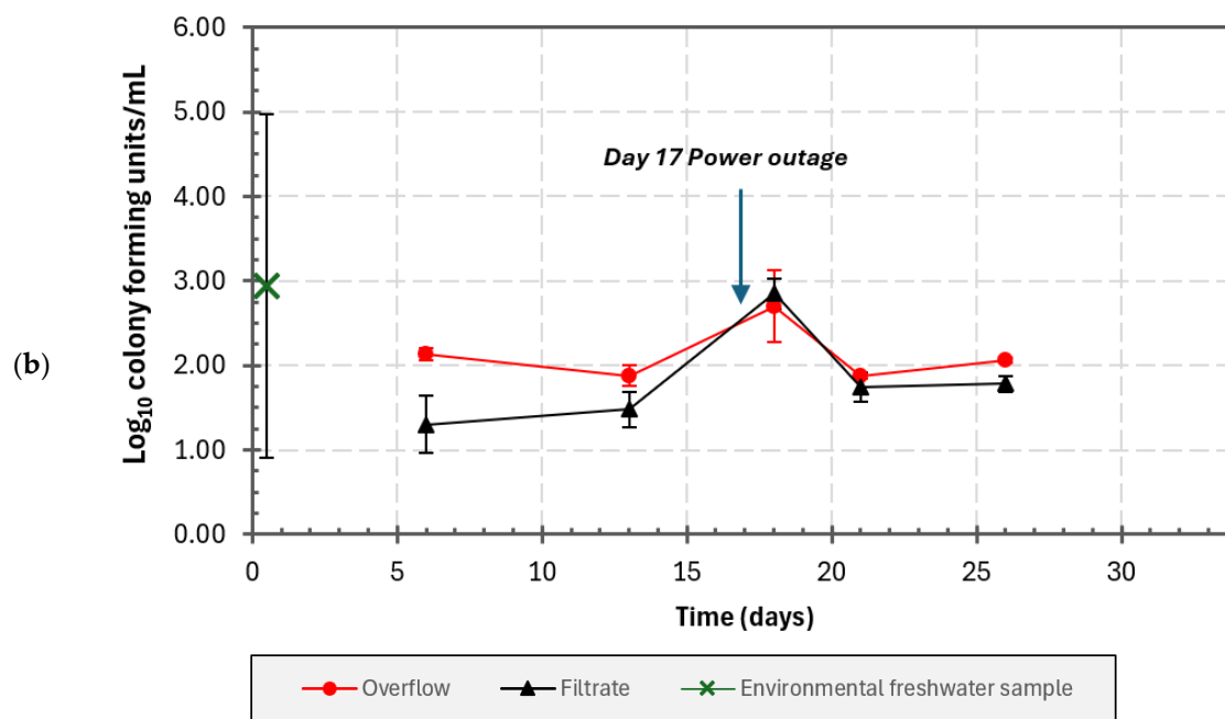
Figure 4. Concentration of bacteria in the overflow and filtrate (heterotrophic plate counts, TSA agar, overnight incubation at 35 \pm 2 °C) for the (a) TSSF and (b) SDSSF. The blue arrow represents the pump failure event outlined in the opening of Section 3.2 (SDSSF only).
