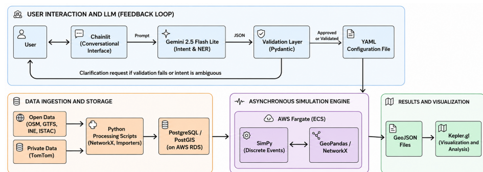
Figure 1. Detailed system architecture highlighting four primary layers: (1) the Conversational AI interface incorporating Gemini 2.5 and Pydantic for validated YAML generation and user feedback loops; (2) Data Ingestion pipelines unifying open and proprietary sources into a PostGIS database; (3) the Asynchronous Simulation Engine powered by SimPy and orchestrated via AWS Fargate; and (4) the output visualization layer using Kepler.gl.
