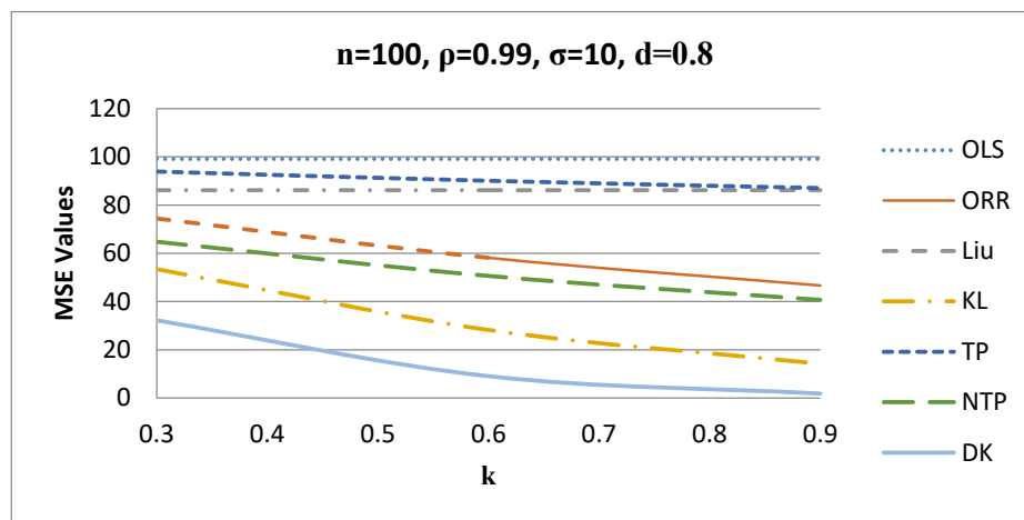
Figure 6. MSE values versus k values when d = 0.8 .
