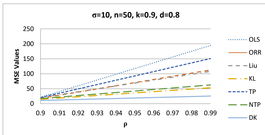
Figure 1. MSE values versus \rho values.
