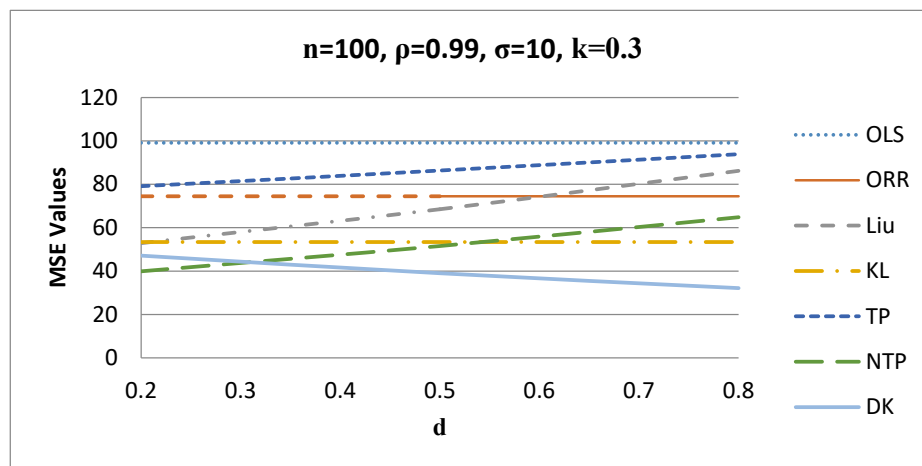
Figure 4. MSE values versus d values when k = 0.3 .
