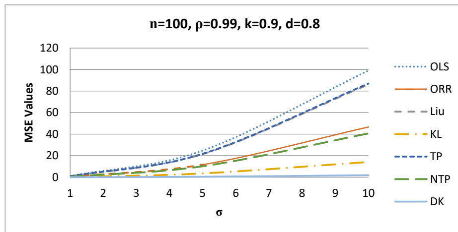
Figure 3. MSE values versus \sigma values.
