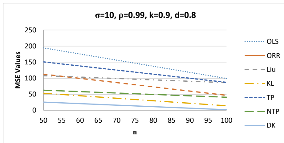
Figure 2. MSE values versus n values.
