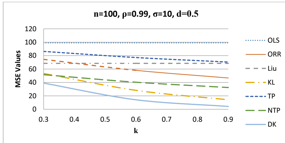
Figure 5. MSE values versus k values when d = 0.5 .
