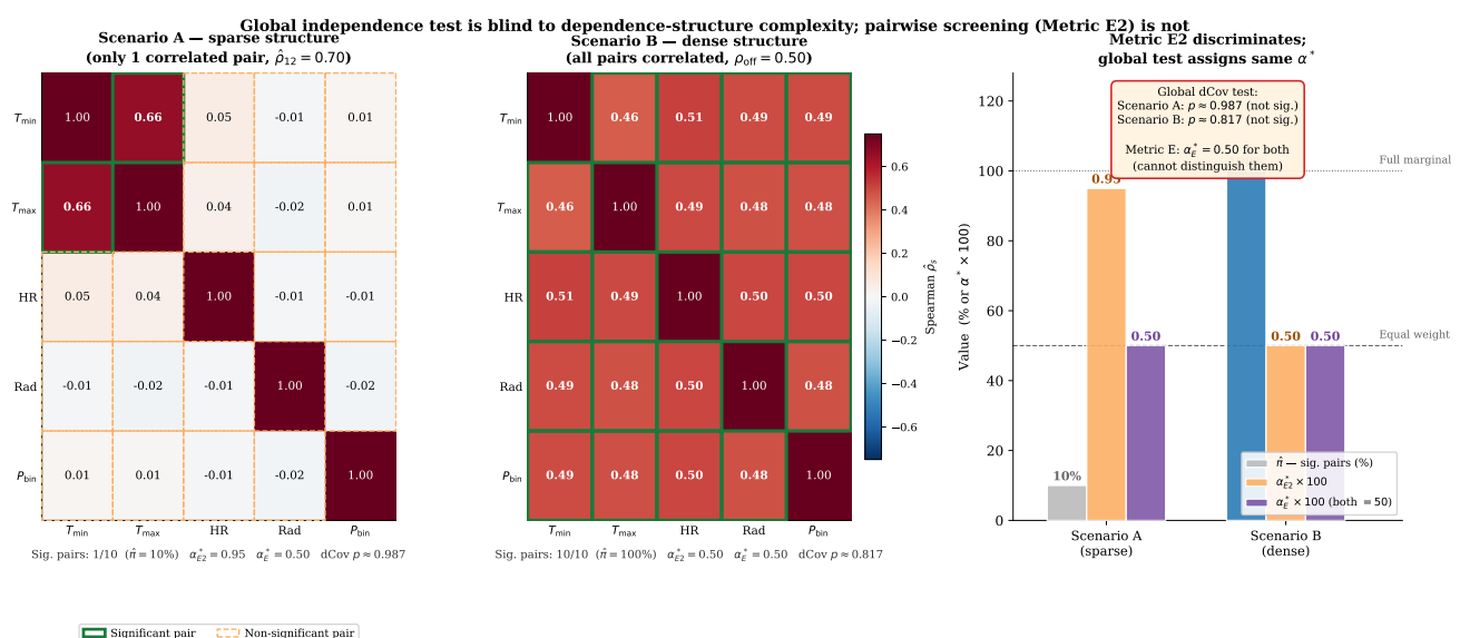
Figure 2. Motivation for Metric E2. (Left and Centre): empirical Spearman correlation matrices for two simulated scenarios ( N = 1000, K = 5 ). Green solid borders mark pairs significant after Holm–Bonferroni correction ( \alpha_{\text{test}} = 0.05 ); orange dashed borders mark non-significant pairs. Scenario A (sparse) has only one significant pair; Scenario B (dense) has all ten pairs significant. (Right): summary of the diagnostic statistics for both scenarios. The global distance-correlation test yields p > 0.05 for both, so Metric E assigns \alpha^* = 0.5 in both cases and cannot distinguish them. The pairwise index \hat{\pi} immediately separates the two structures.
