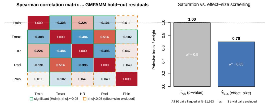
Figure 4. Pairwise Spearman test results for the Valle del Cauca hold-out. (Left): Spearman correlation matrix of standardised GMFAMM hold-out residuals ( N_{test} \approx 31,663 ). Cell values give \hat{\rho}_s ; at this sample size, all ten pairs are significant under Holm–Bonferroni correction. (Right): the effect-size screening ( |\hat{\rho}_s| \geq 0.05 ) excludes the three pairs with negligible correlation ( T_{min}-P_{bin} , HR-P_{bin} , Rad-P_{bin} ), yielding \hat{\pi}_{0.05} = 0.70 and \alpha_{E2}^* = 0.65 , versus the saturated significance-based \hat{\pi}_{sig} = 1.0 ( \alpha_{E2}^* = 0.50 ).
