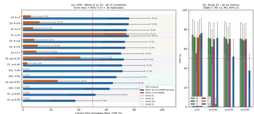
Figure 3. (a): Correct Discrimination Rate (CDR) for Metric E (orange) and Metric E2 (blue) across all 15 simulation conditions (M1 vs. M3). Error bars show 95% confidence intervals ( \pm 1.96\sqrt{p(1-p)/30} ); differences < 2 SE ( \approx 9 pp) should be interpreted cautiously. Red dashed line = 50% chance level. Conditions ordered by E2 CDR descending; coloured strip indicates the study. Metric E falls below 50% in 7 of 15 conditions; Metric E2 remains above 50% in 14 of 15 conditions. (b): CDR for all six metrics (A–E2) in Study S1 (M1 vs. M3), reproduced from Table 7 with 95% CI shown. Studies S2, S2b, and S3 were specifically designed to compare E vs. E2 and did not evaluate A–D; the full six-metric comparison is therefore shown only for Study S1. Metrics A, B, and D maintain positive discrimination across all \rho levels; Metric E inverts the ranking from \rho \geq 0.40 ; Metric E2 degrades only at \rho = 0.90 (see also Supplementary Figure S1).
