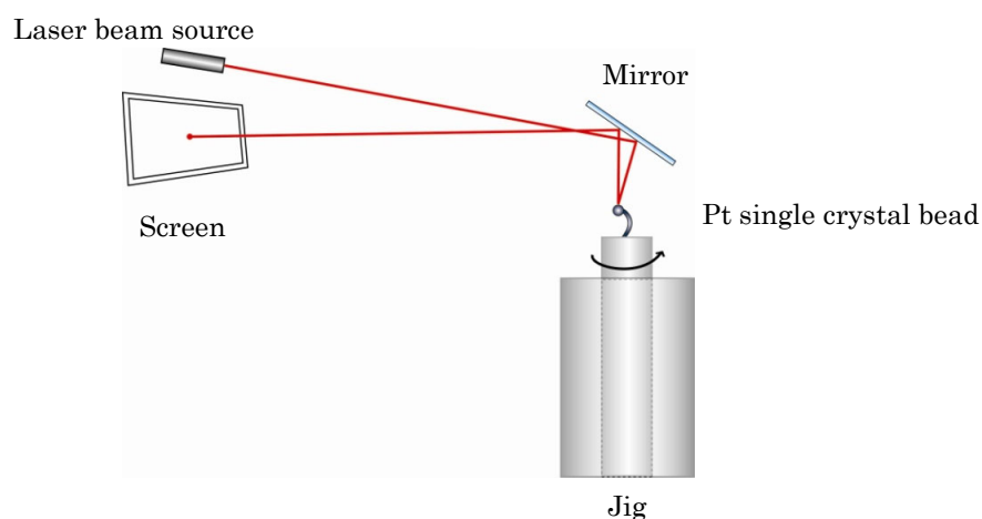
Figure S1 Schematic illustration of the adjustment of (111) and (100) facets by a laser beam reflection method
