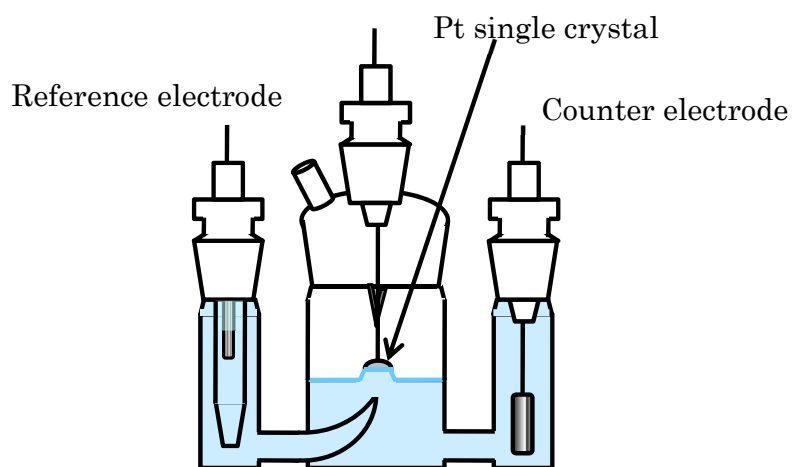
Figure S2 Schematic illustration of a three-compartment cell. The electrochemical measurements were carried out with the hanging meniscus method.
