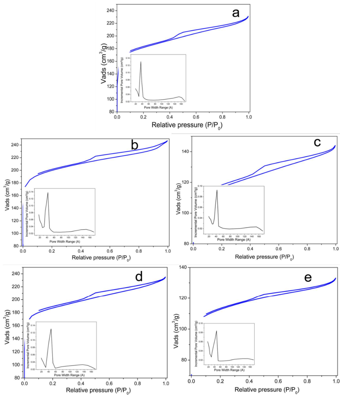
Figure 1. Nitrogen adsorption/desorption isotherm and DH pore size distributions of raw AC (a), acid treated AC (b), WC/AC (c), 1%Pt/AC (d) and 1% Pt-WC/AC samples (e).
