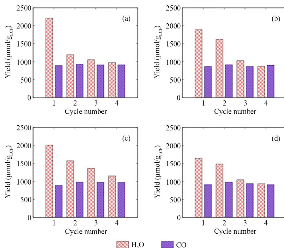
Figure 6. RWGS-CL results of LCF synthesized by the ball milling method calcined at different temperatures: (a) no calcination, (b) 800 °C, (c) 950 °C, and (d) 1050 °C.
