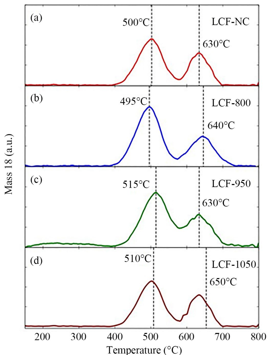
Figure 4. H 2 -TPR results of LCF synthesized by the ball milling method calcined at different temperatures: (a) no calcination, (b) 800 °C, (c) 950 °C, and (d) 1050 °C.
