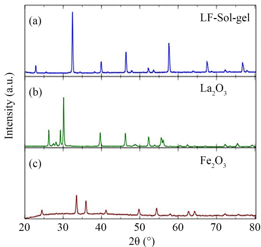
Figure 2. XRD results of referenced samples: (a) LaFeO 3 made by sol-gel; (b) La 2 O 3 made by calcinating La(NO 3 ) 3 ·6H 2 O; (c) Fe 2 O 3 made by calcinating Fe(NO 3 ) 3 ·9H 2 O.
