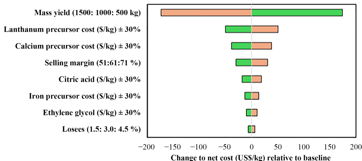
Figure 8. Sensitivity analysis for the synthesis of LCF synthesized by the Pechini method. Baseline catalyst cost of US$ 486.97 per kg of catalyst. 2021 is considered the basis year. The orange bar represents the high value, and the green bar represents the lower value.
