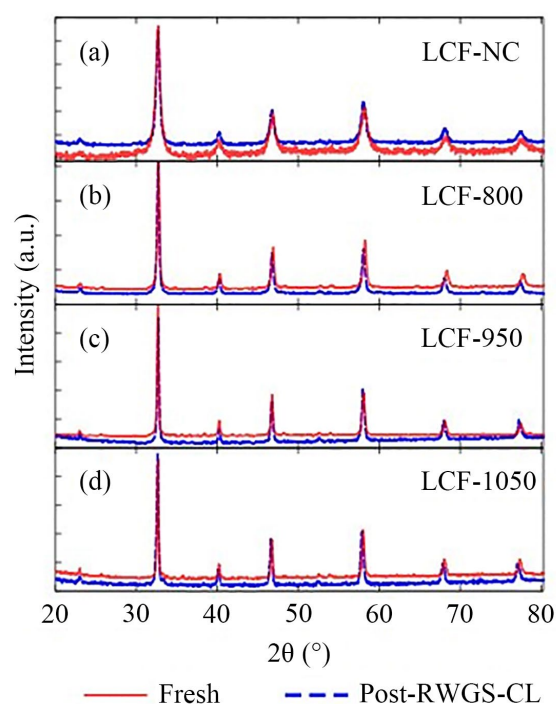
Figure 1. XRD results of ball-milling synthesized LCF using metal oxide precursors and calcined at different temperatures: (a) no calcination (NC), (b) 800^\circ\text{C} , (c) 950^\circ\text{C} , and (d) 1050^\circ\text{C} .
