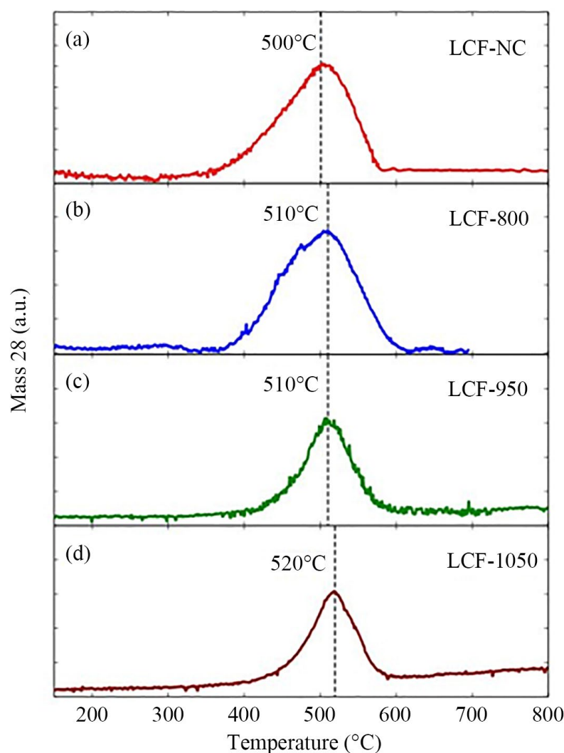
Figure 5. CO 2 TPO results of LCF synthesized by the ball milling method calcined at different temperatures: (a) no calcination, (b) 800 °C, (c) 950 °C, and (d) 1050 °C.
