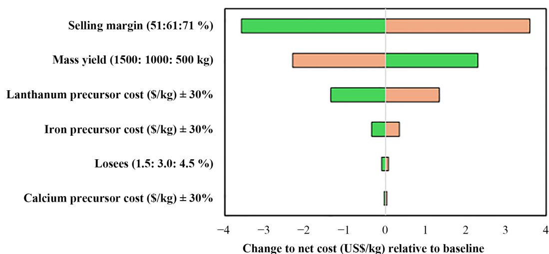
Figure 7. Sensitivity analysis for the synthesis of LCF synthesized by ball milling. Baseline catalyst cost of US$ 57.78 per kg of catalyst. 2021 is considered the basis year. The orange bar represents the high value, and the green bar represents the lower value.
