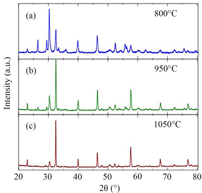
Figure 3. XRD patterns of LF synthesized by ball milling using nitrate precursors and calcined at different temperatures: (a) 800 °C; (b) 950 °C; (c) 1050 °C.
