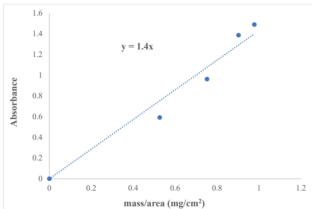
Figure 2. Calibration plot for O-H stretching peak for CNFs at 1060 cm -1 .
