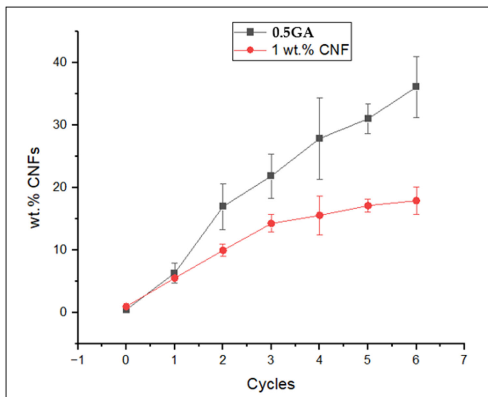
Figure 3. wt.% CNFs for 0.5GA and 1 wt.% CNF suspensions as a function of pressing cycles. The error bars represent the standard deviation from three separate trials.
