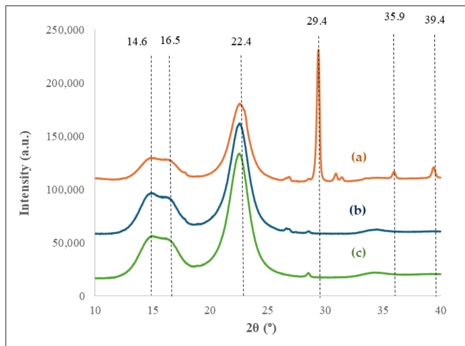
Figure 8. XRD patterns for (a) dewatered 0.5GA suspension, (b) rehydrated 0.5GA suspension after GCC removal, (c) original supplied 3 wt.% CNF suspension.
