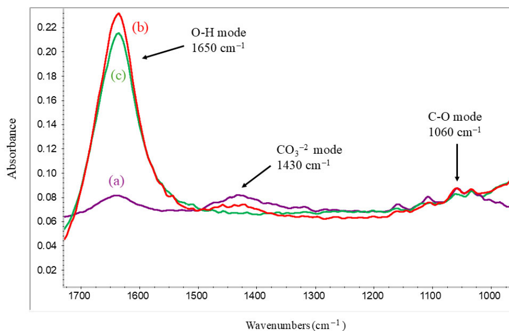
Figure 4. IR spectra for (a) the dewatered 0.5GA suspension and the 0.5GA suspensions after acid washing with (b) 2 mL HCl/1 g GCC and (c) 2 mL HCl/100 mg GCC. The key bands in this spectrum have been indexed.
