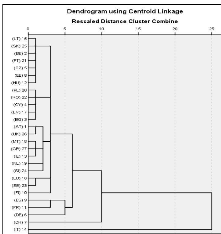
Figure 5. The dendrogram of EU countries eco-innovation performances in 2013.
