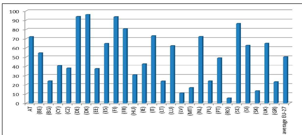
Figure 2. The mean score of ECO-INNOVATION INDEX in the EU-27 countries.
