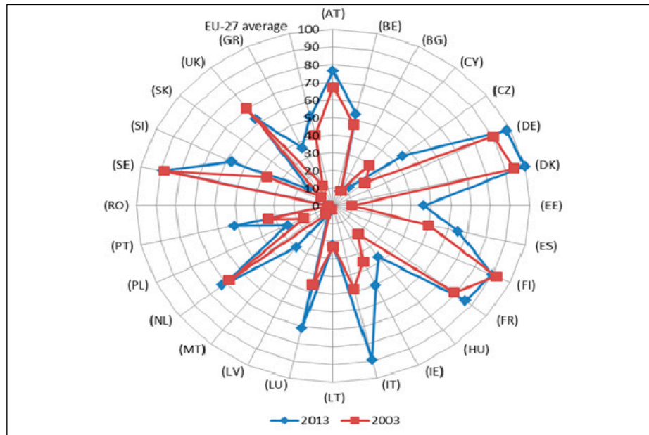
Figure 3. The level of ECO-INNOVATION INDEX in 2003 and 2013 for EU countries.
