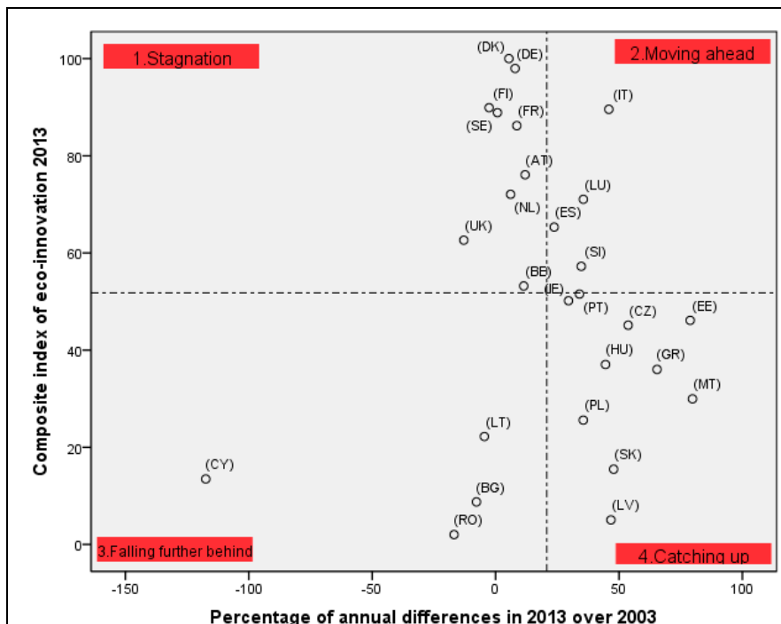
Figure 4. Overall country trends by ECO-INNOVATION INDEX.
