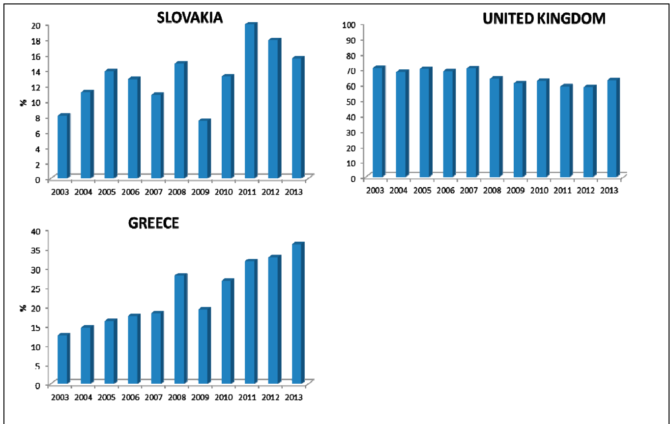
Figure 1. The ECO-INNOVATION INDEX during the period 2003–2013 in the 25 EU countries.
