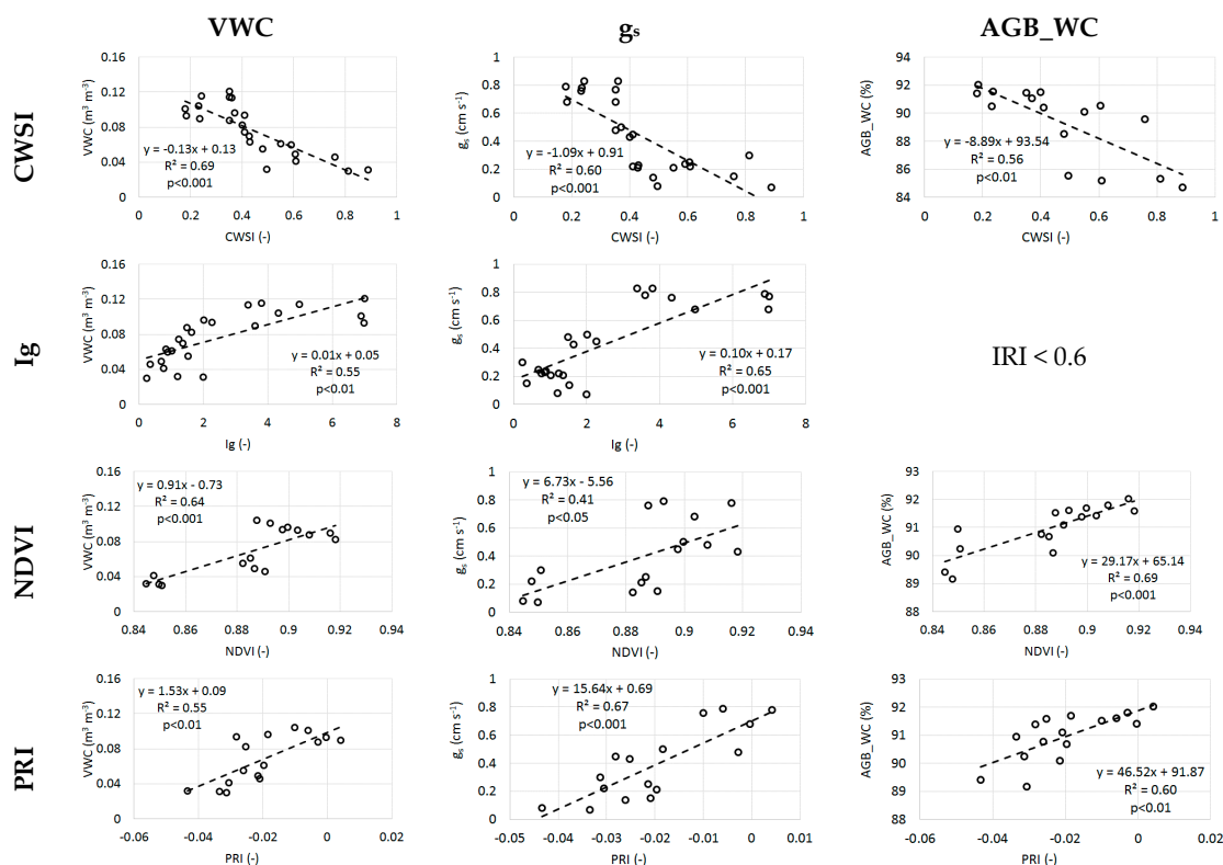
Figure 6. Linear regression models between thermal ( CWSI and I_g ) and optical ( NDVI and PRI ) indices, and reference variables ( VWC , g_s and AGB_WC ) describing the crop water status. Data are from the EX2 campaign.
