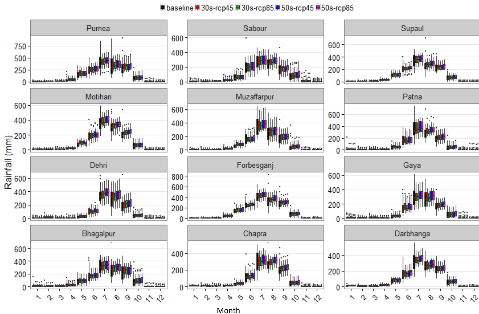
S1. Box plot of monthly rainfall amounts in the baseline period (1908-2009) and in 2030 and 2050 under two emission scenarios (rcp4.5 and rcp8.5) at 12 stations in Bihar, India.
