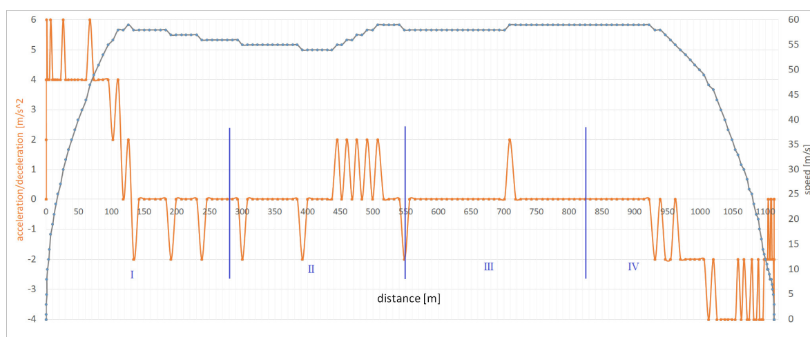
Figure 5. Train movement diagram (source: own elaboration).
