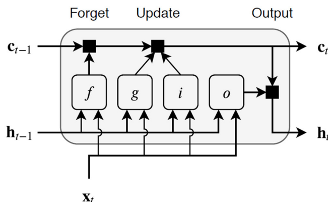
Figure 4. LSTM block structure (source: [36]).
