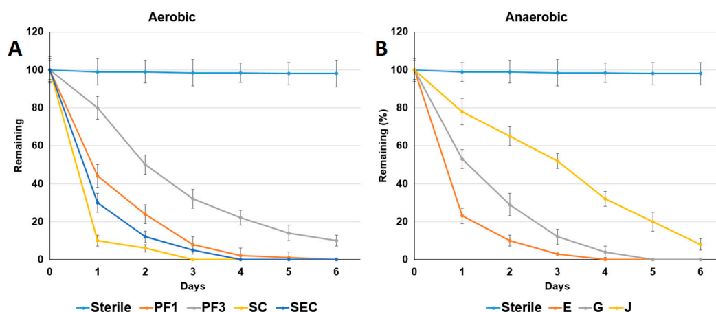
Figure 2. Comparison of the acetaminophen degradation abilities of the isolated bacterial strains. (A) Bacterial strains PF1, PF3, SC and SEC (without sediments) under aerobic conditions; (B) bacterial strains E, G and J (without sediments) under anaerobic conditions. Sterile: sterilized medium without the addition of bacteria. GS: Guandu sediment. BS: Bali sediment. GSterile: sterilized Guandu sediment. BSterile: sterilized Bali sediment. Data from three independent experiments are presented as the means \pm SE.
