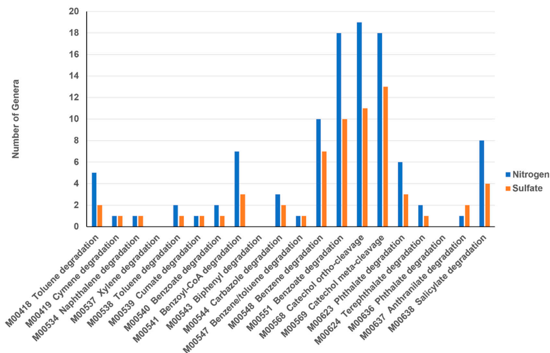
Figure 11. Distributions of number of major microbial genera with different aromatic compound degradation pathways. Mxxxxx are KEGG database module ID. Nitrogen: 30 major microbial genera identified in the experiments using electron acceptors that are associated with nitrogen metabolism. Sulfate: Major 30 microbial genera identified in the experiments using electron acceptors that are associated with sulfate–sulfur metabolism.
