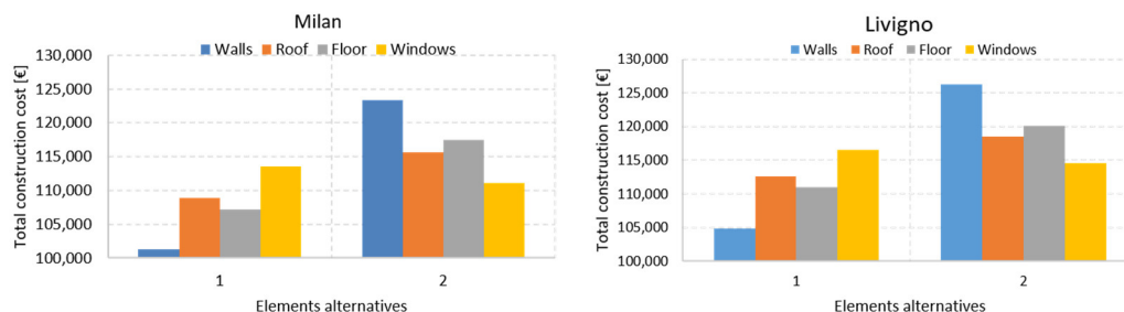
Figure 8. Construction cost according to building component typologies.
