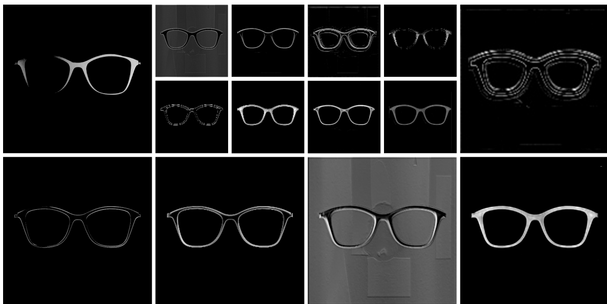
Figure 13. Examples of the intermediary steps our CNN takes for processing a sample.
