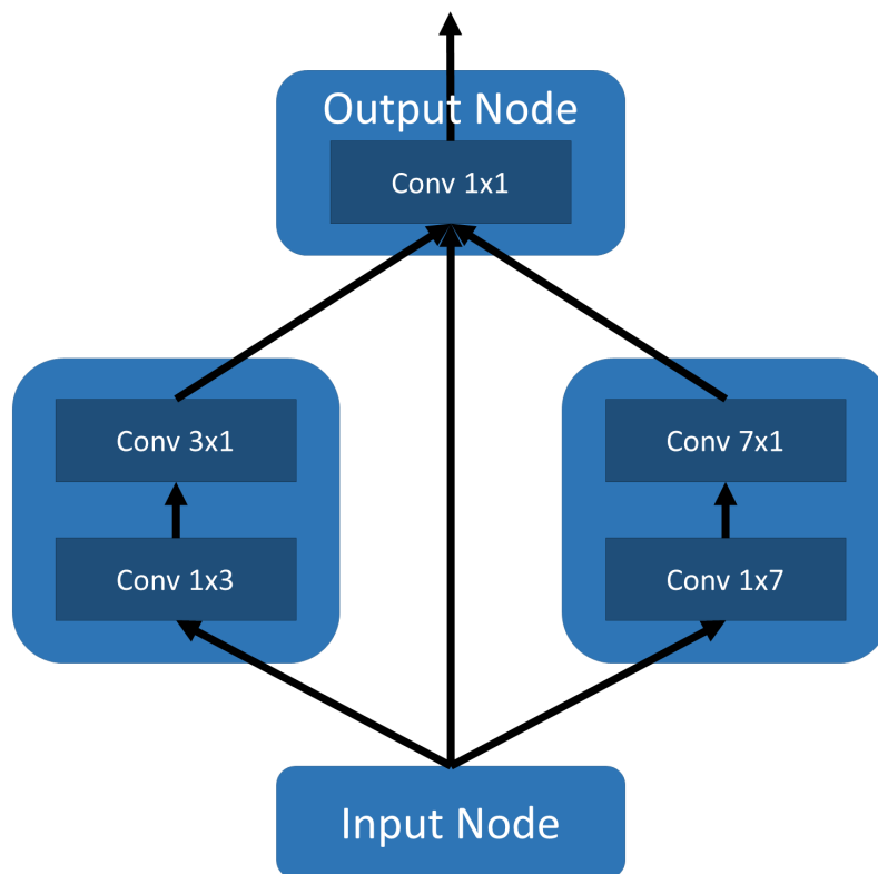
Figure 11. Discovered CNN cell.
