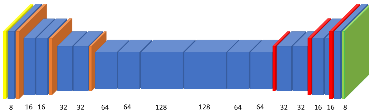
Figure 10. Network used for evaluation on datasets consisting of larger images.
