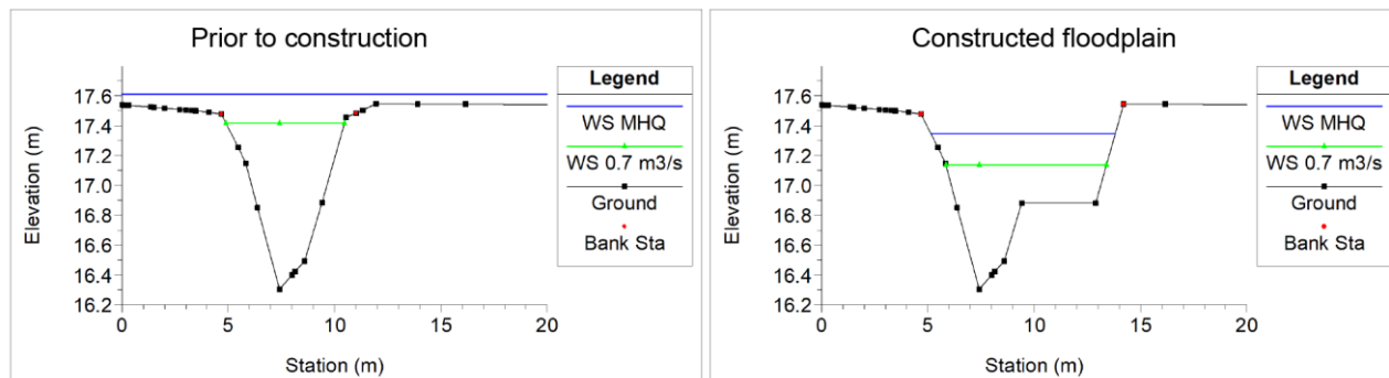
Figure 2. A representative channel cross-section before ( left ) and after two-stage channel construction ( right ), with simulated water surface levels (WS) at a 1-in-5 year flow ( 1.6 \text{ m}^3/\text{s} ) and a more frequent ( 0.7 \text{ m}^3/\text{s} ) flow event during spring conditions.
