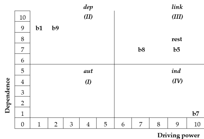
Figure 2. Driving–dependence power diagram for OSC barriers.
